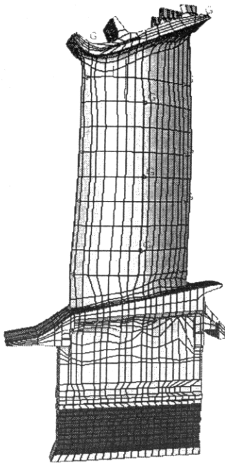
Fig. 1 FE model of the rotor blade
