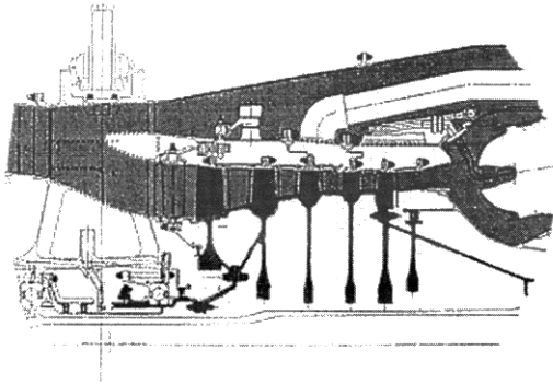
Figure 2: EJ200 5-Stage HP-Compressor, Schematic Cross Section
