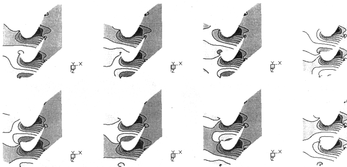
Fig. 4 Instantaneous pressure distributions at mid-height of the rotor blade
