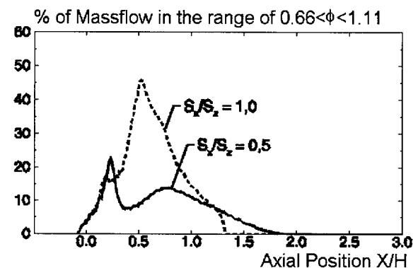
Fig. 4.8: Effect of S_x/S_z ratio on the mixing when heat release is considered
