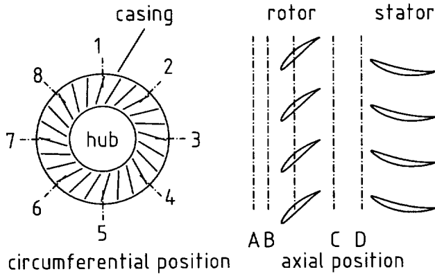
Figure 6: Probe locations and blade sections at mid-span
