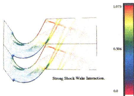
Figure 22 : Illustration of Shock Resolution Possible with Fine Zero Exit Angle Grids - Relative Mach No. Contours.
