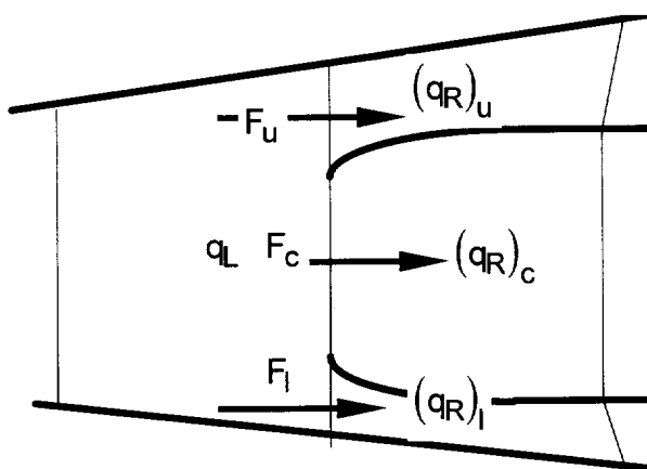
Figure 6: Straight-flow flow-division
