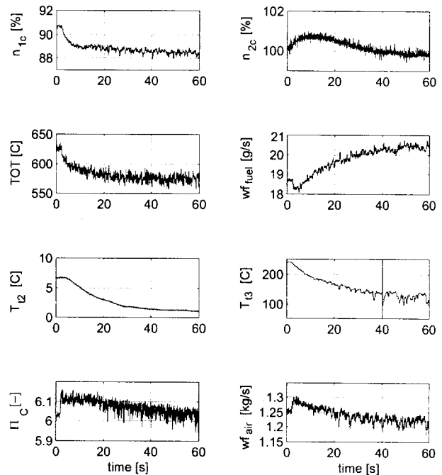
Figure 13: Engine parameters during water ingestion
