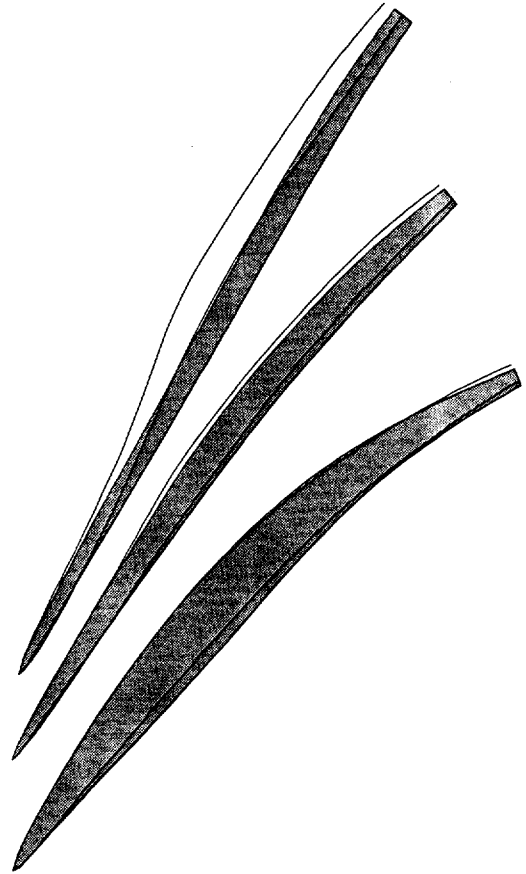
Fig. 9 : Initial (grey) and modified blade geometry at hub, mean and shroud
