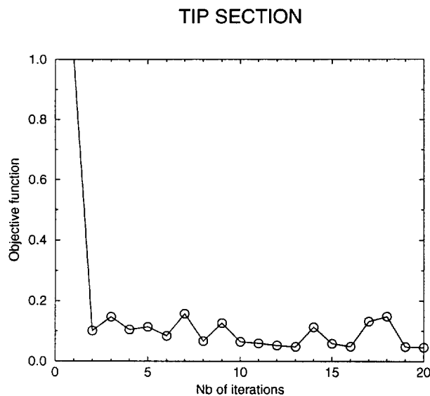
Fig. 9 : Design convergence history
