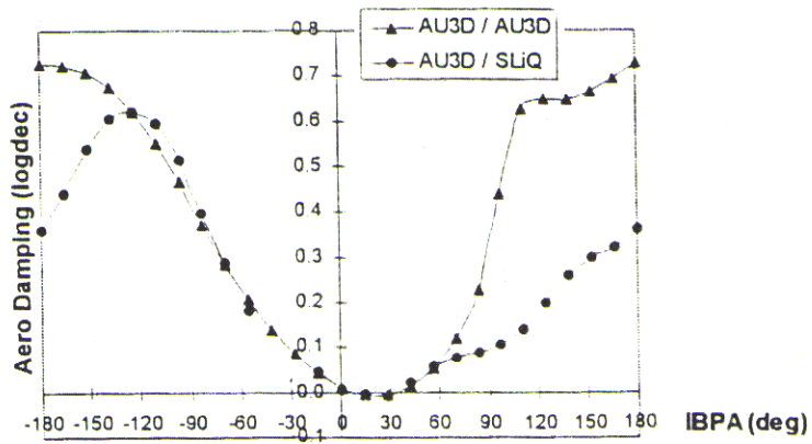
Figure 3: Stability analysis results, wide chord fan blade
