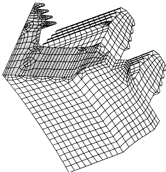
Figure 10. Crack plane after smoothing.
