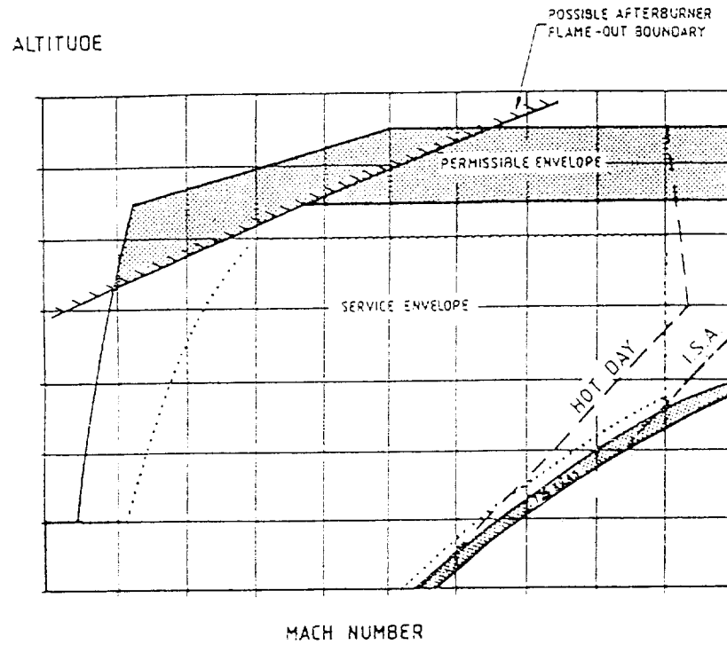
Fig. 1 - Engine Flight Envelope
