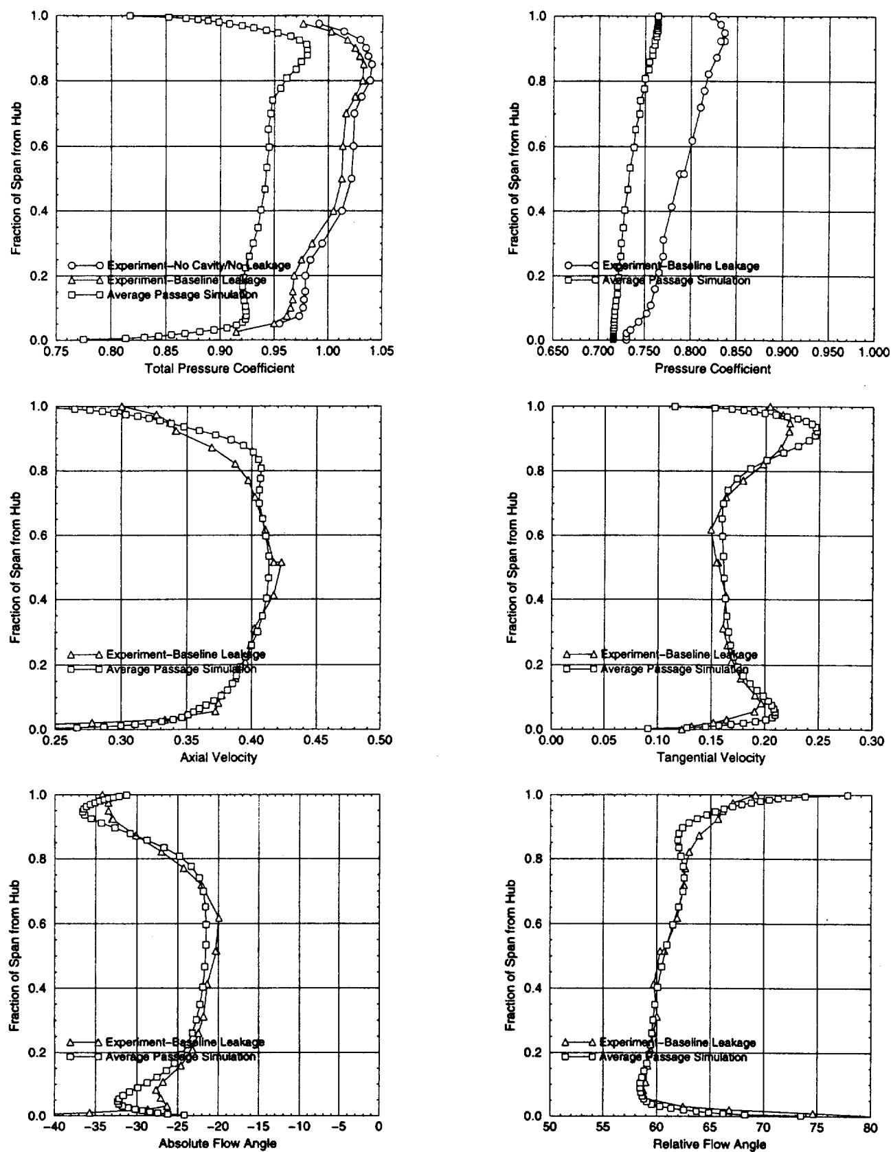
Fig. 4. Axisymmetric flow variables at Station 3.0.
