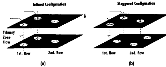
Fig. 4.2: Inlined and staggered mixer configurations
