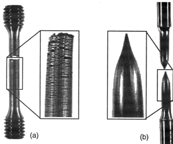
Fig. 6: Environmental embrittlement of an \text{Ti}_3\text{Al} base alloy (Ti-25Al-10Nb-3V-1Mo) during tensile testing at 700^\circ\text{C} ; (a) tested in air, (b) tested in vacuum.
