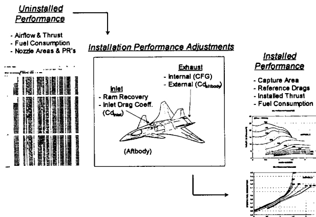
Figure 8 - Engine Installation Process
