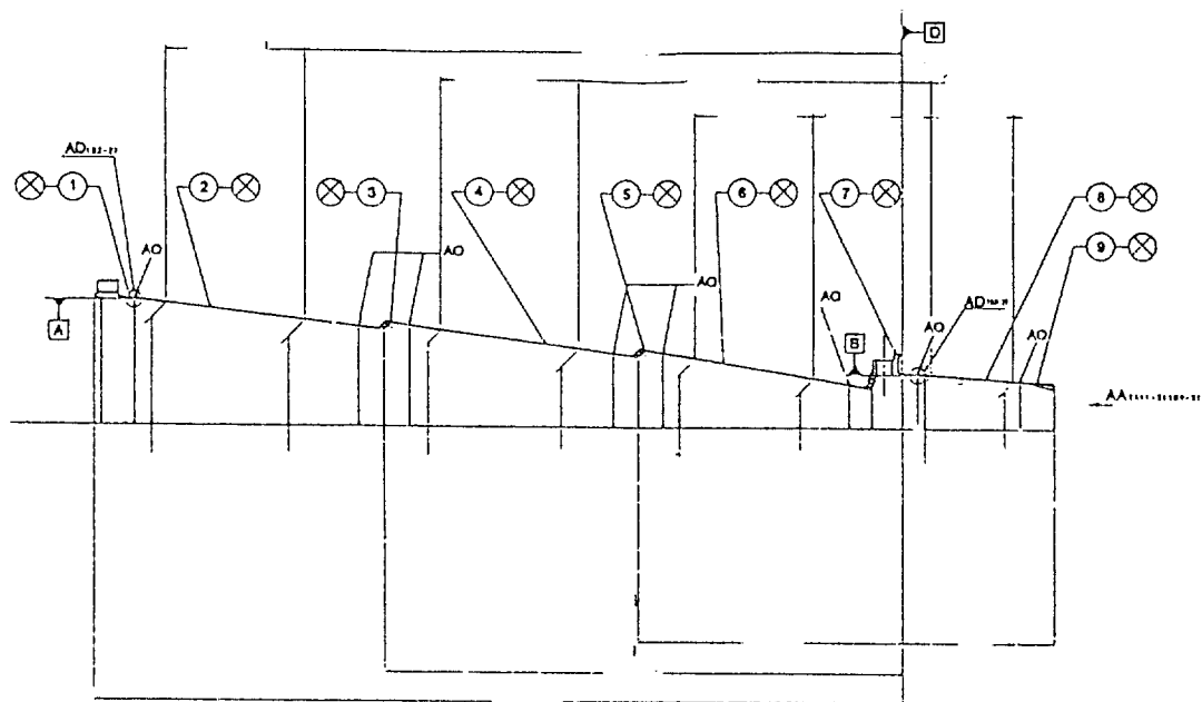
Fig. 7b - Heat Shield Original Design
