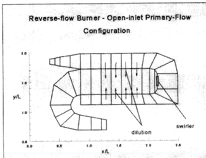
Figure 5: Discretization of a reverse-flow combustor
