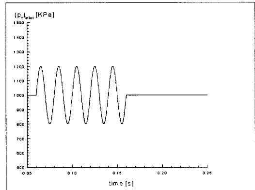
Figure 20: Oscillations in inlet p_t
