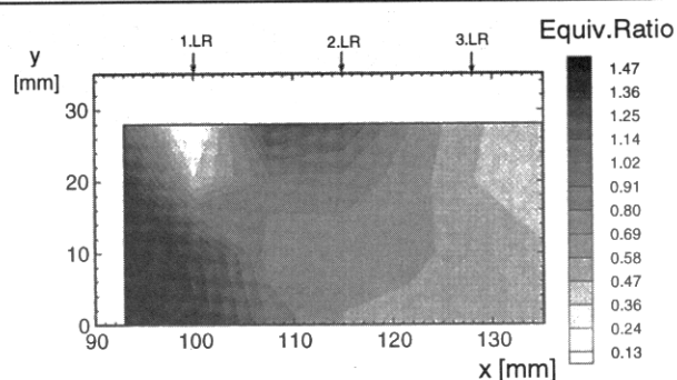
Fig. 4.10: Chemically reacting mixing field
