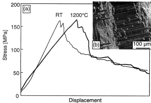
Fig. 18: Ceramic Matrix Composite (CMC): (a) strain/elongation plot of Nextel 720/mullite composite (b) fracture surface.
