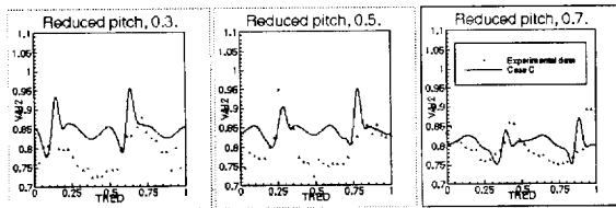
Figure 9 - Midspan unsteady evolution of the reduced absolute velocity.
