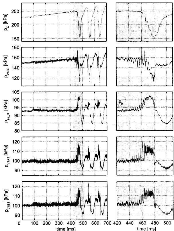
Figure 11: Surge during moderate acceleration
