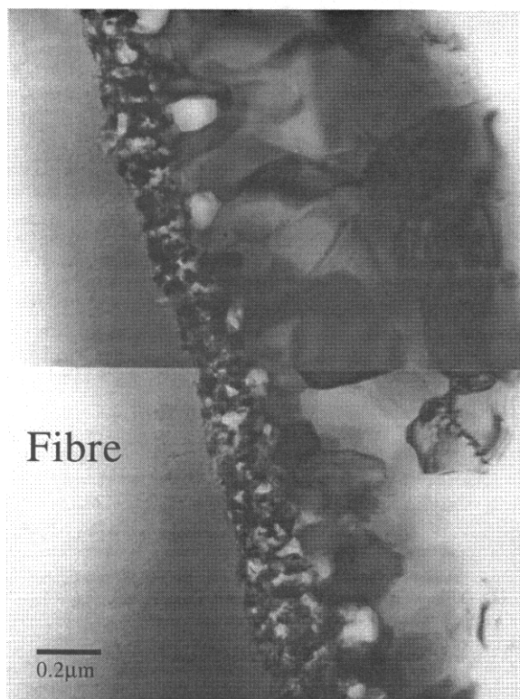
Figure 11 TEM Image of Fibre Matrix Interface
