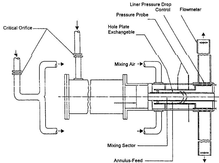
Fig.3.1: Scheme of experimental rig
