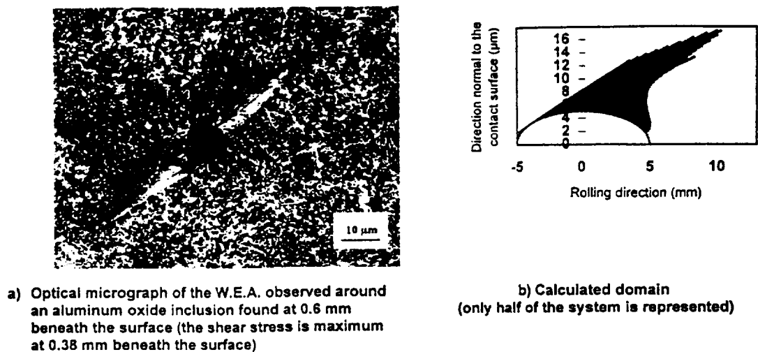
Figure 2 : Comparison between an experimental W.E.A. and the corresponding calculated domain swept by dislocations ( P_H = 4.5 GPa ; 52 100 steel)
