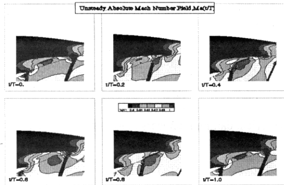
Figure 12 - Unsteady flow field, Mach number.
