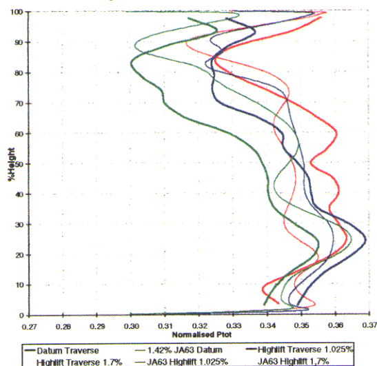
Figure 23 : Radial Variation of Normalised Absolute Total Pressure Ratio - Datum and Highlift Rotor Close Exit Plane (~111mm)
