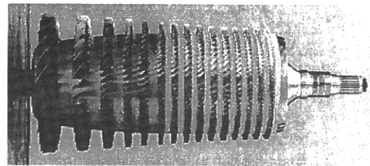
Figure 5: 15-stage compressor for stationary gas turbine application
