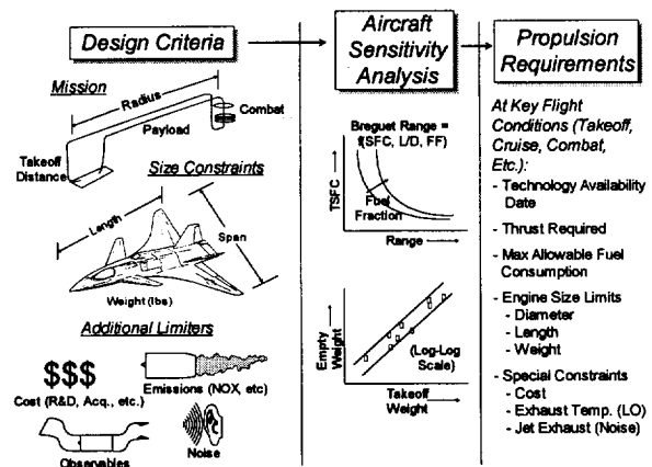
Figure 3 - Propulsion Requirements Definition
