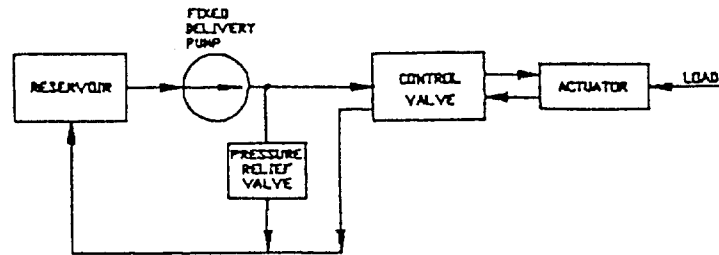
a – Valve controlled system – fixed delivery pump
