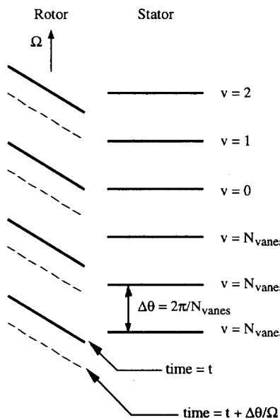
Figure 3. Rotor moves one stator passage in t = \Delta\theta/\Omega
