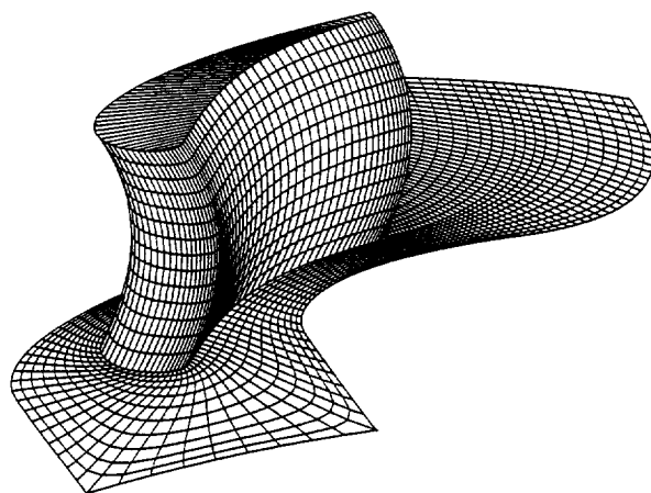
Fig. 11 : 3D view of the leaned blade
