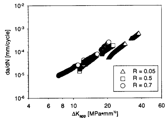
Figure 4: da/dN vs. \Delta K_{app} for René 95 at 400°C.
