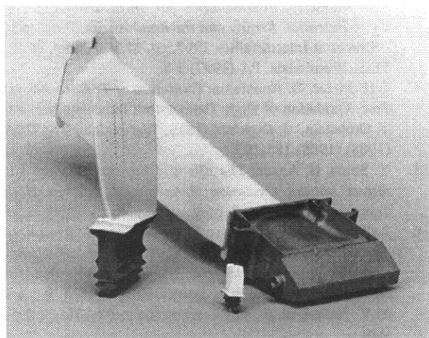
Fig. 16: EB-PVD TBCs on aircraft engine and stationary gas turbine blades.
