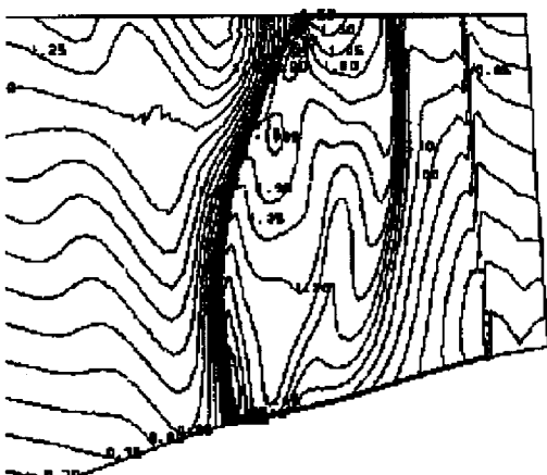
Figure 12: Predicted Mach Number Distribution, Blade Suction Side
