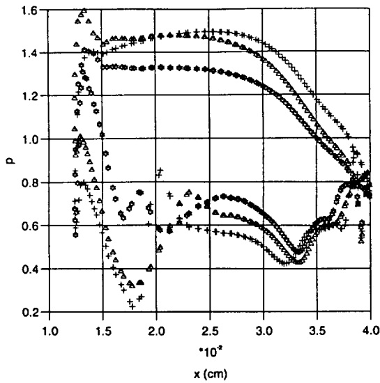
Fig. 12 Instantaneous rotor static pressure profiles
