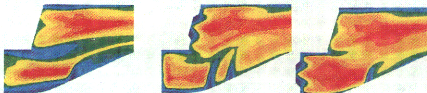
TEMPERATURE MAPS AT 3 DIFFERENT SECTIONS
