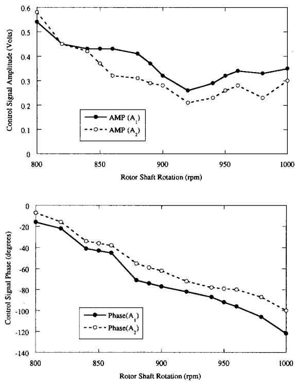
Figure 13. Control signal voltage amplitude and phase as a function of rotor shaft rotation
