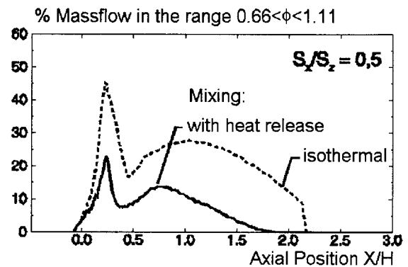
Fig. 4.7: Effect of heat release on the mixing
