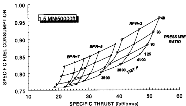
Figure 6 - GSA Uninstalled Performance Trades
