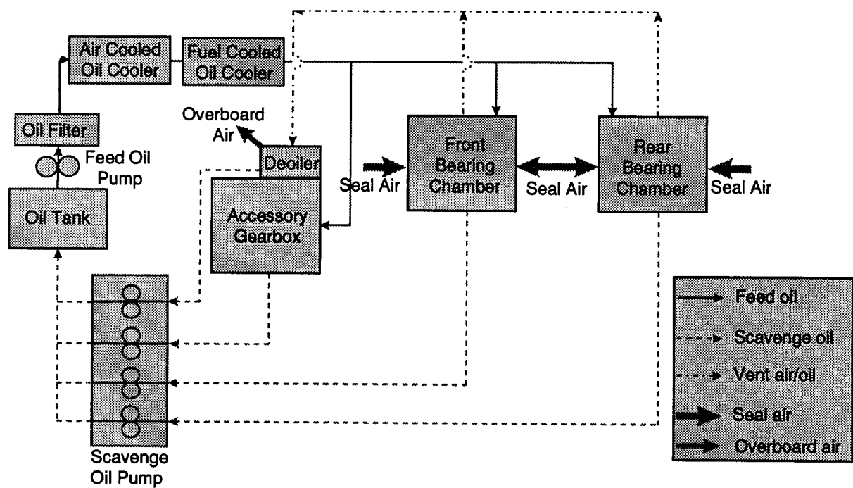
Figure 2: Simplified Lubrication Oil System
