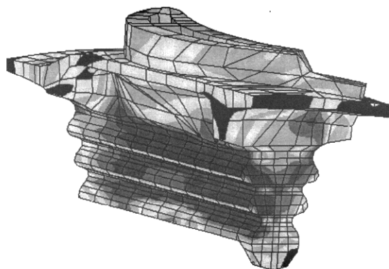
Blade fixing
