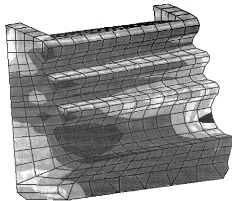
Disc fixing
