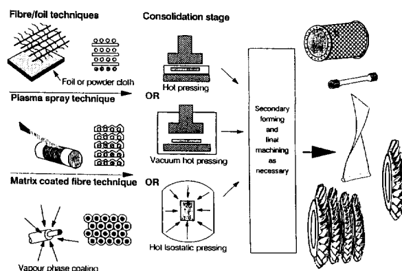
Figure 4 Manufacturing Routes for TMC
