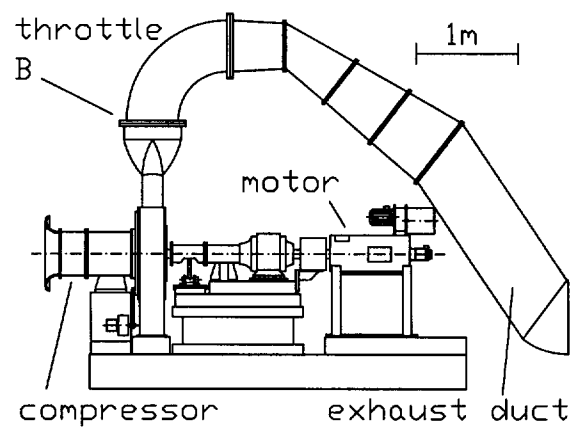
Figure 4: Overview of the test stand
