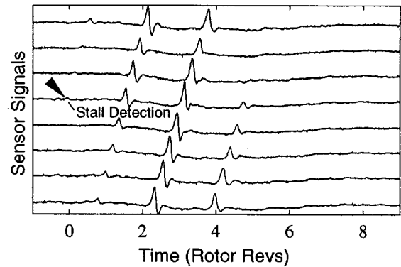
Figure 19: Stall evolution with the modified two-step controller
