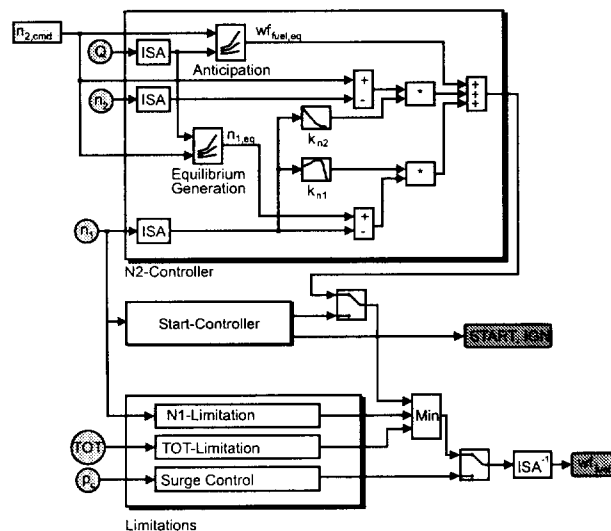
Figure 4: Schematic of the engine control
