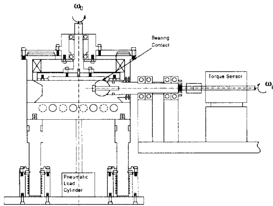
Figure 2. Cross section of the Rolling Contact Friction Tester. Rotations of the disk shaft and ball shaft are depicted by \omega . The torque sensor measures the friction in the bearing contact under a combination of rolling and sliding conditions. Load is applied to the bearing contact through the pneumatic cylinder.
