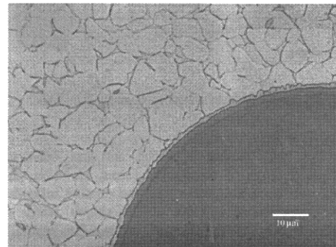
Figure 9 As Processed Ti-6Al-4V/SCS-6 Composite
