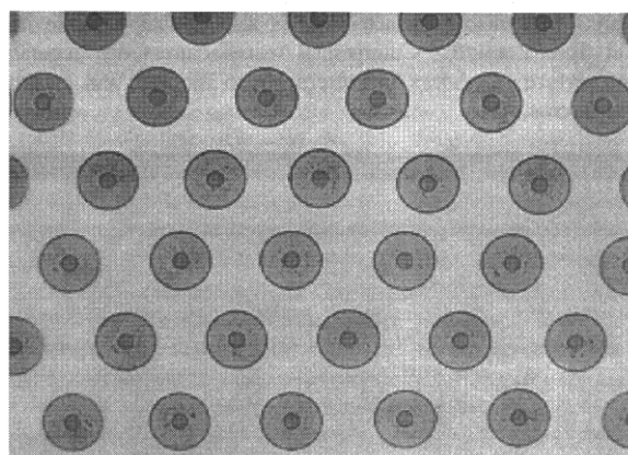
Figure 6 MCF Fibre Distribution
