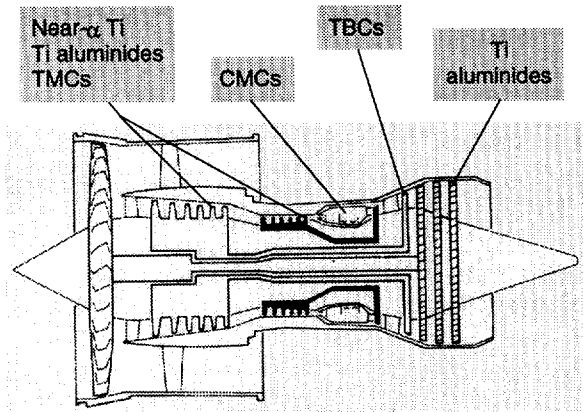
Fig. 1: Schematic allocations of advanced materials technologies and aircraft engine components leading to significant payoff.
