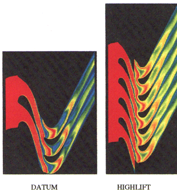
Figure 28: Entropy Contours Illustrating the NGV Wake Motion through the Rotor Passage.
