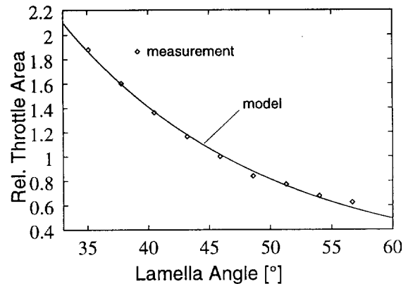
Figure 16: Characteristic of the dynamic throttle
