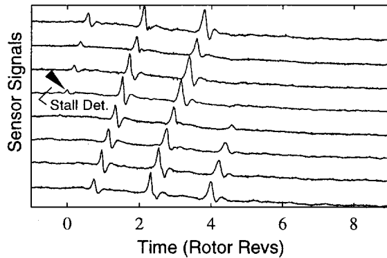
Figure 18: Stall evolution with the two-step controller
