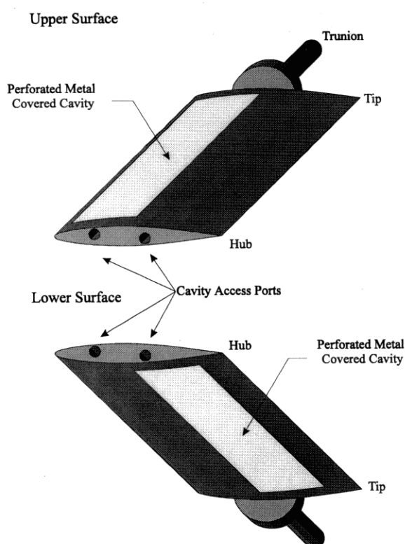
Figure 8. Active stator airfoil
