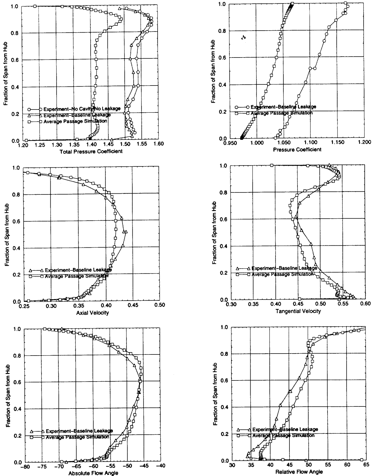
Fig. 5. Axisymmetric flow variables at Station 3.5.
