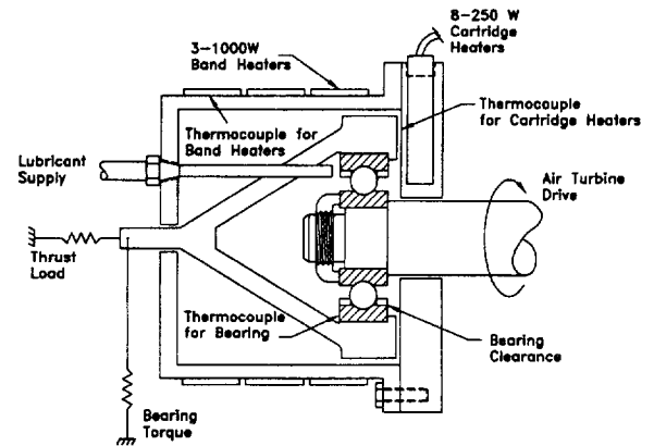
Figure 3. Cross section of the High Speed Bearing Tester. The shaft speed is controlled by an air turbine drive. The vapor delivery system was connected to the tube labeled lubricant supply. The bearing temperature was taken from the thermocouple mounted to the bearing outer race.
