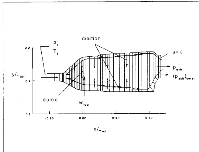
Figure 9: Straight-flow burner - Configuration and discretization
