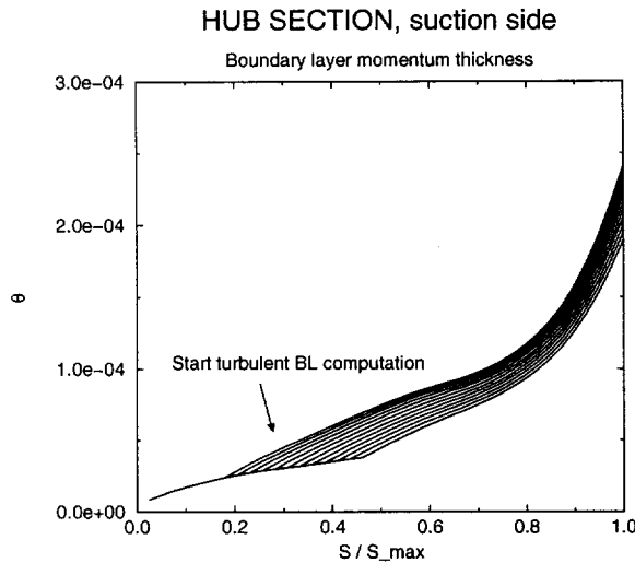
Fig. 12 : Boundary layer momentum thickness (suction side)
