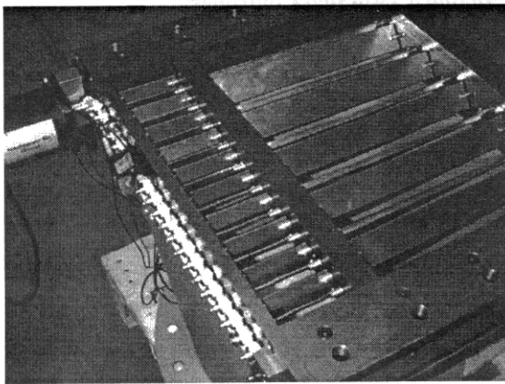
Figure 14: The dynamic throttle
