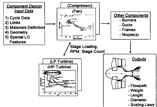
Figure 10 - Generalized Engine Component/Flowpath Design
