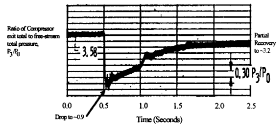
Figure 12. Test Data: Ratio of Compressor Exit Total Pressure to Free Stream Total Pressure (Choby, et al., 1971)
