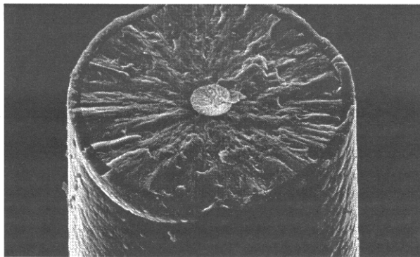
Figure 8 SiC Fibre Growth Defect
