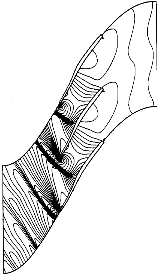
Fig. 8 : Iso-density lines at shroud of the redesigned transonic compressor rotor
