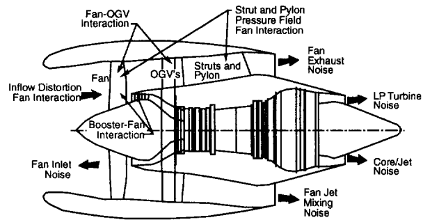
Figure 1. Sources of turbomachine noise
