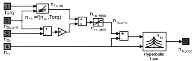
Figure 22: Generation of set points for the acceleration
