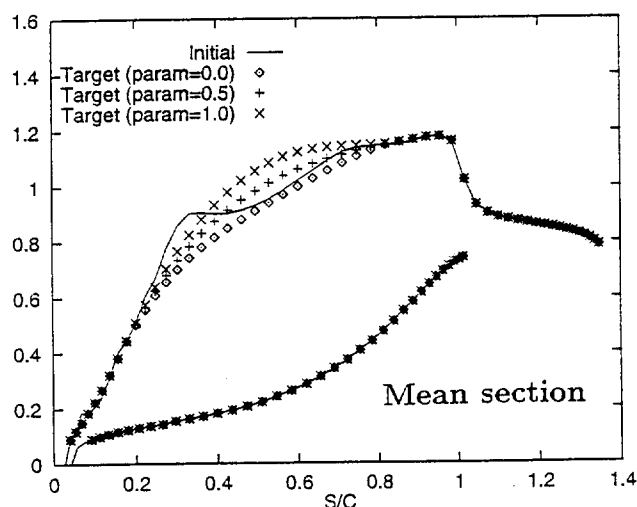
Fig. 12 : Initial and prescribed is. Mach number distributions at mean section
