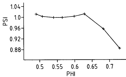
Figure 7: Characteristic of the stable operating regime
