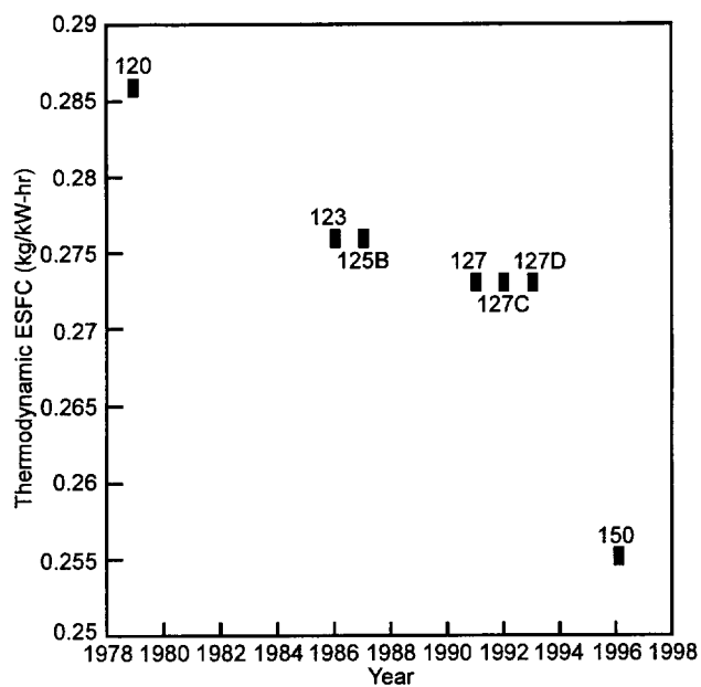
Fig. 4 PW100 fuel consumption evolution
