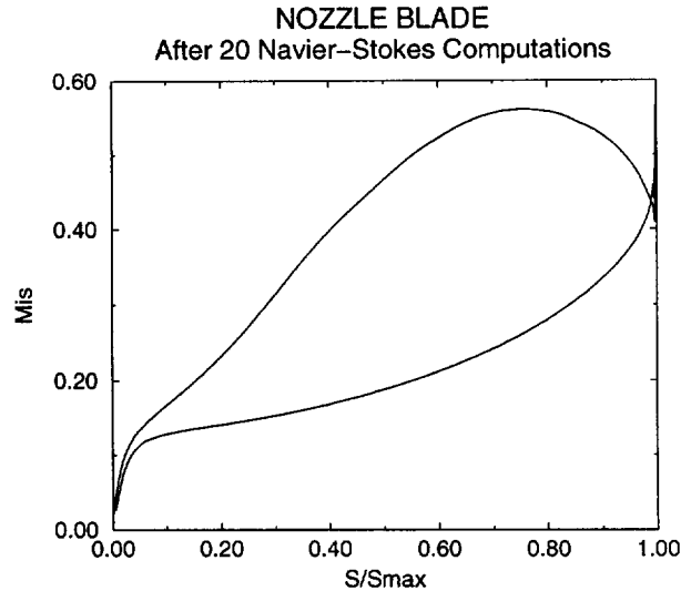
Fig. 17 : Mach number distributions on the blade surface
