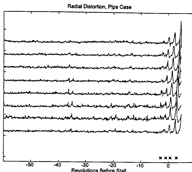
Figure 1. Pressure Traces for Radial Distortion
