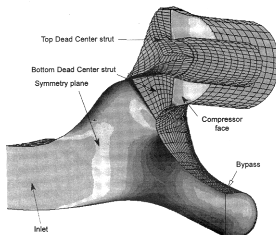
Fig. 8 PW100 inlet system
