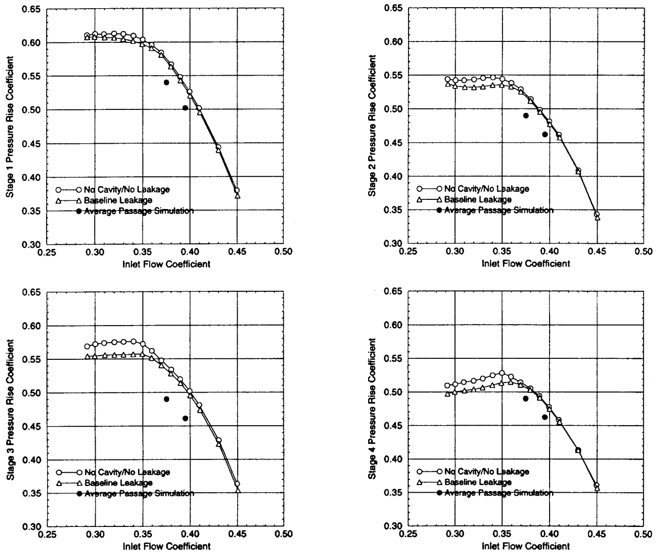
Fig. 2. Individual stage pressure rise coefficient as a function of inlet flow coefficient.
