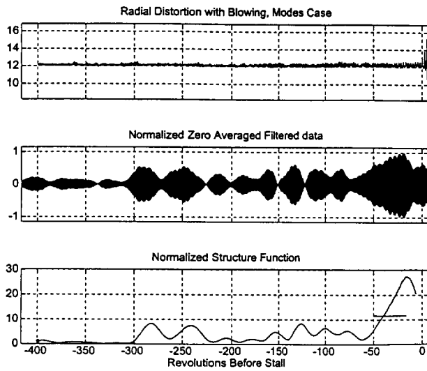
Figure 7. Structure Function Results Radial Distortion With Injection
