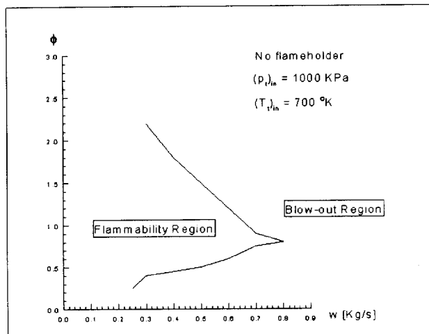
Figure 15: Constant-area duct - Blowout limits
