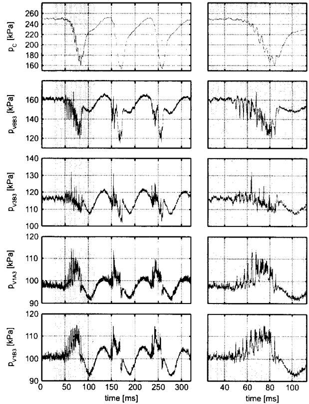
Figure 7: Surge caused by throttling at quasi steady state conditions
