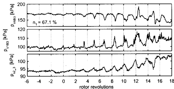
Figure 15: Pressure signals for stall detection
