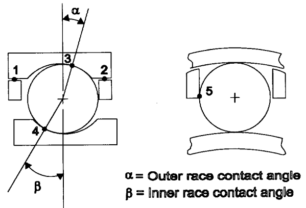
Figure 8. Contacts in a ball bearing: (1) Outer Race / Cage-land 1 (2) Outer Race / Cage-land 2 (3) Outer Race / Rolling element contact (4) Inner Race / Rolling element contact (5) Rolling element / Cage contact.
