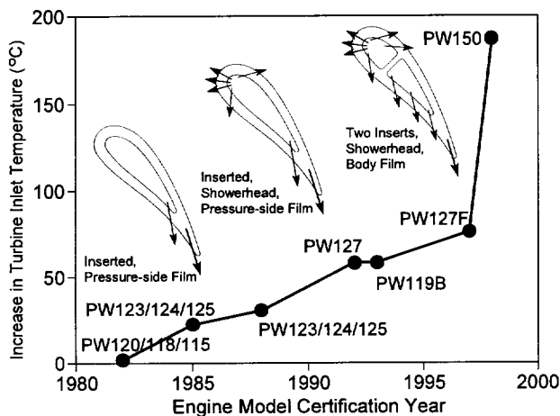
Fig. 16 Evolution of PW100 turbine inlet temperature
