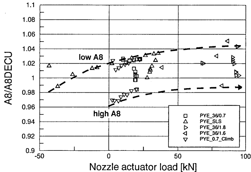
Fig. 15b Deviation between the analysed nozzle area A_8 and the control system input A_{8,DECU} correlated with nozzle actuator load
