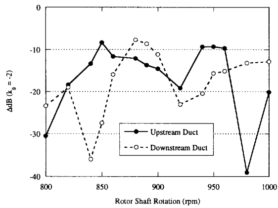
Figure 12. Control authority over wide range of operating conditions
