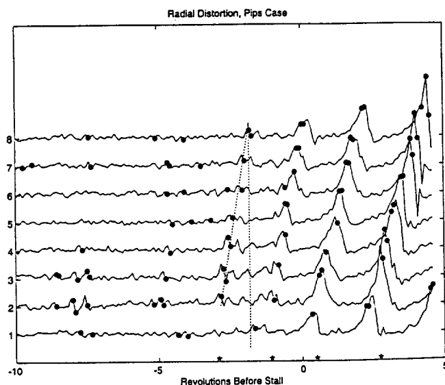
Figure 2. Pressure Traces 10 Revolutions Before Stall
