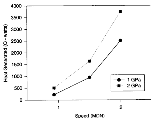
Figure 9. ADORE heat generation values predicted at speeds of 0.97, 1.5, and 2.0 MDN with inner race Hertzian stresses of 1 and 2 GPa
