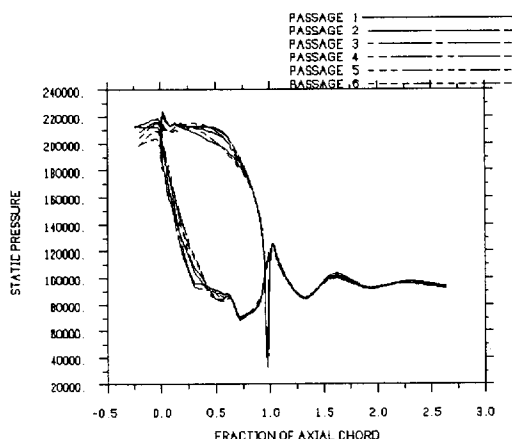
Figure 21 : Highlift Mid-Span Unsteady Static Pressure Plots
