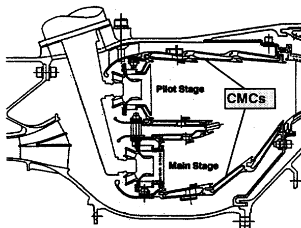
Fig. 17: Advanced combustor design with CMC shingles [51].
