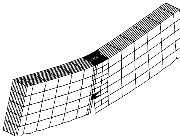
Figure 13. Mesh of the initially cracked structure
