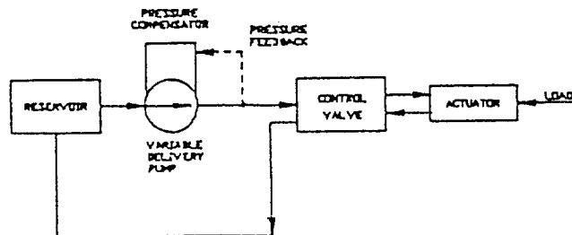
b – Valve controlled system – variable delivery pump – constant pressure
