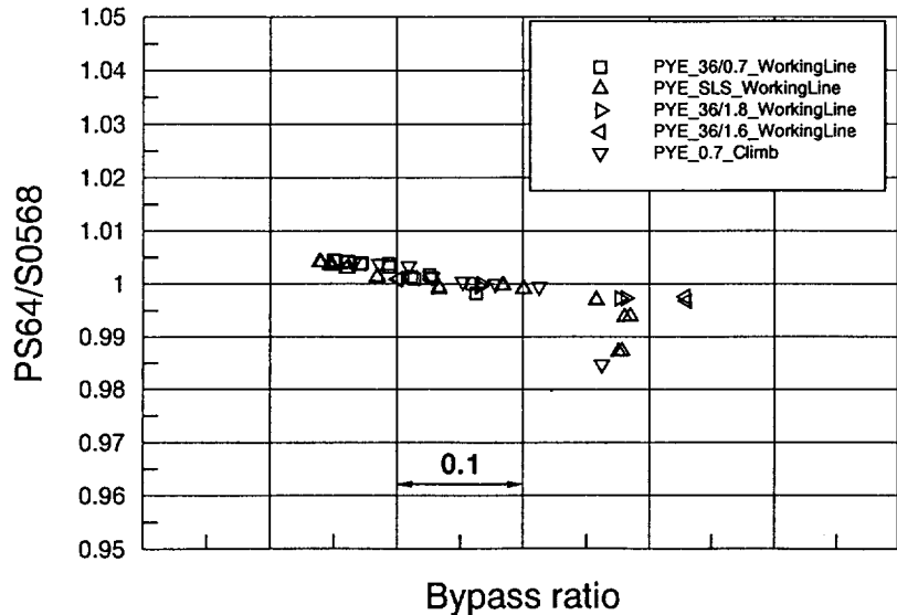
Fig. 12 Correlation between the calculated mixer pressure P_{64} and the measured pressure S0568 (on the liner) in dry operation
