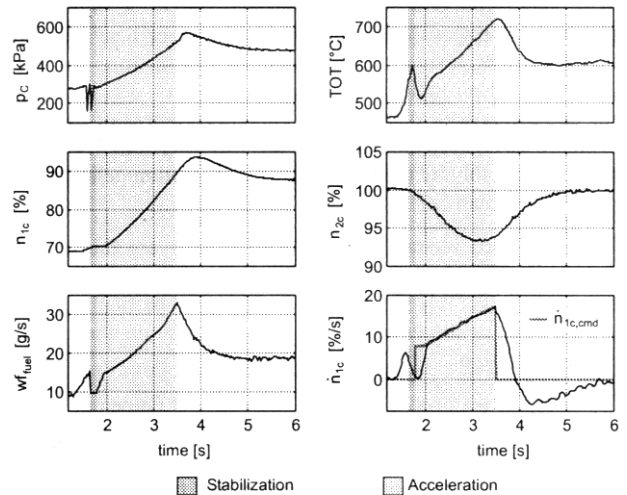
Figure 25: Example of a surge recovery
