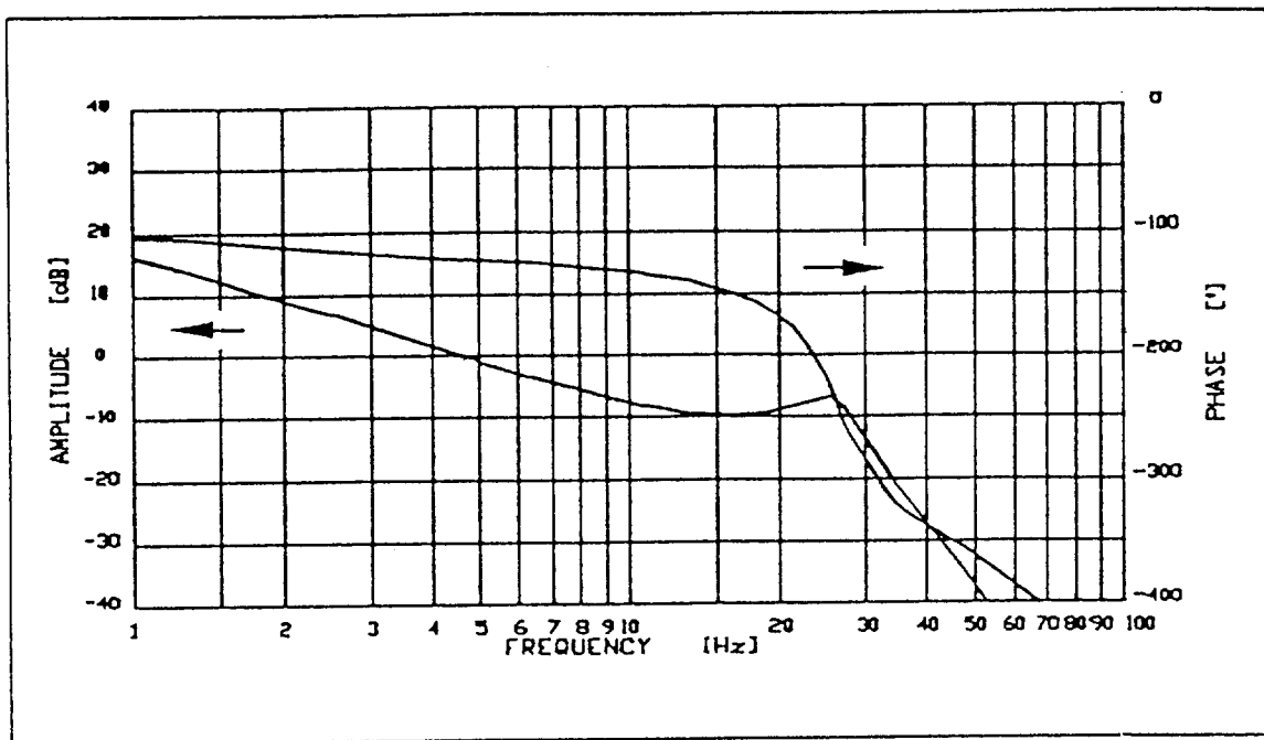
Fig. 12a - VACU : Open Loop Frequency Response at Maximum Pressure
