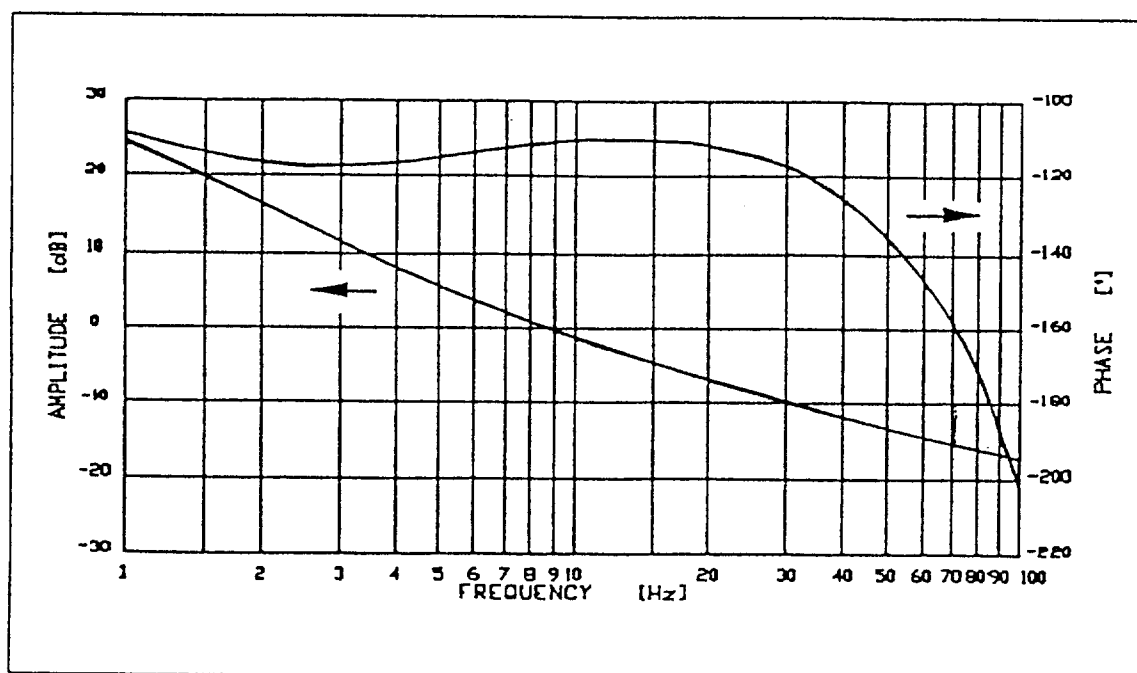
Fig. 9a - NACU Servoloop : Open Loop Frequency Response at Maximum Pressure
