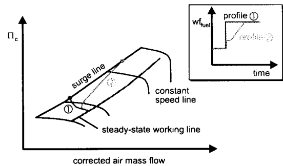
Figure 10: Fuel profiles to bring the engine in surge condition
