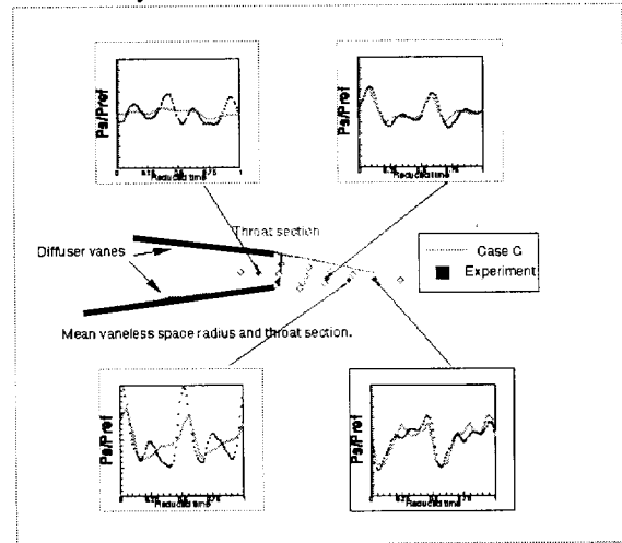
Figure 10 - Confrontation of pressure evolutions.
