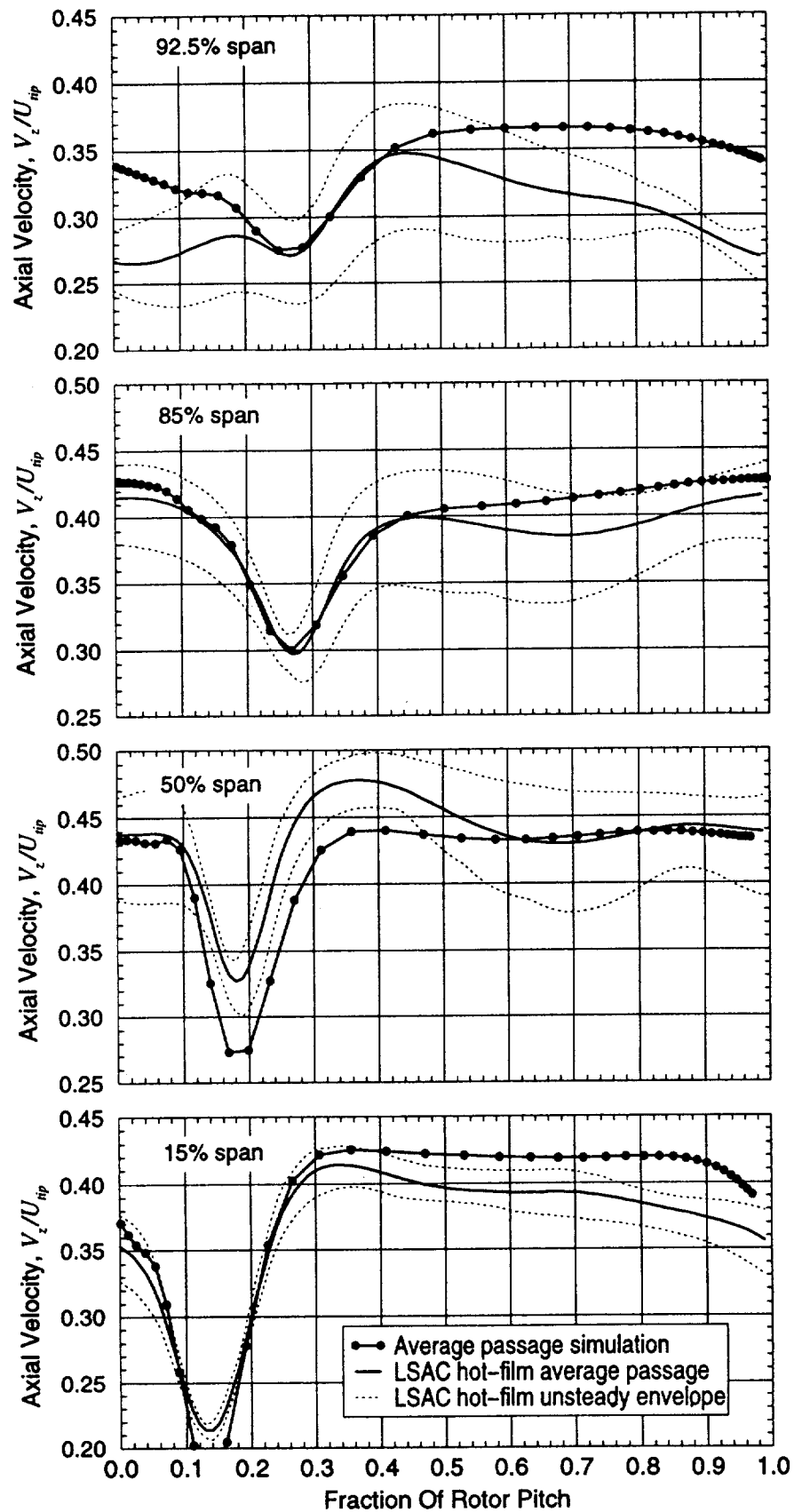
Figure 9. Measured and simulated LSAC axial velocity ( V_z/U_{tip} ) distributions at ST 3.5 for 15, 50, 85 and 92.5% span. Simulation data are denoted by filled circles, average passage data are represented by solid lines and the unsteady envelope data are depicted by dotted lines.
