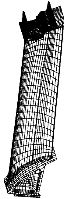
Figure 5. Turbine blade mesh.
