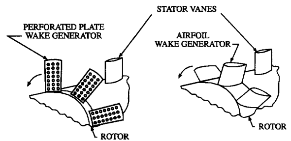
Figure 5. Rotor and stator and representative gust.
