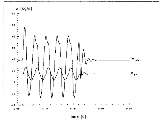
Figure 21: Effect in mass flow-rates
