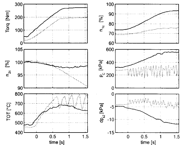
Figure 16: Parameters for surge detection
