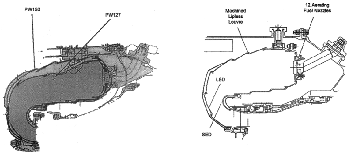
Fig. 12 PW150 combustor compared to PW127
