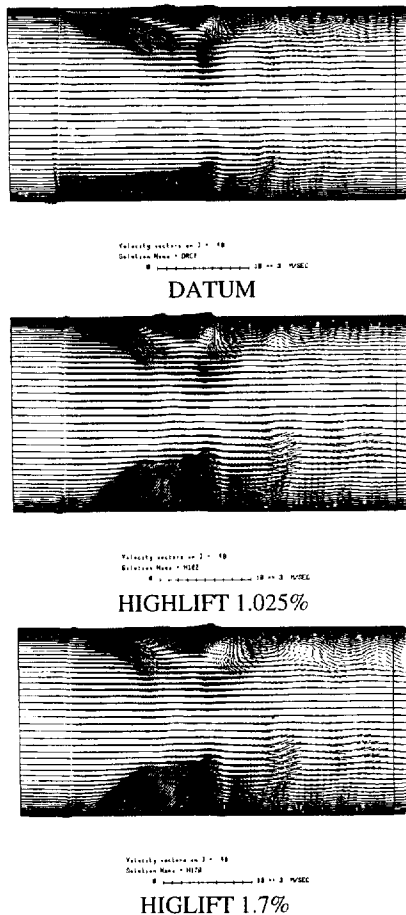
Figure 14 : Vector Diagrams on the Rotor Suction Surfaces.
