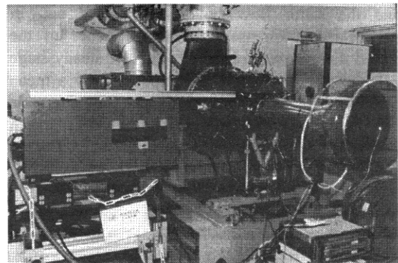
Figure 1- SUPAERO compressor test rig.
