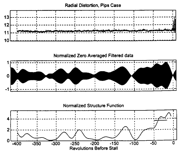
Figure 6. Structure Function Results Radial Distortion
