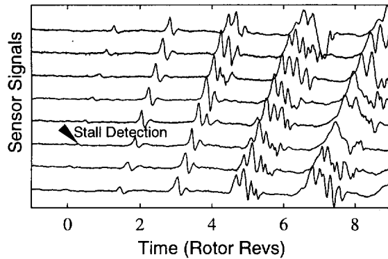
Figure 17: Stall evolution with no controller response
