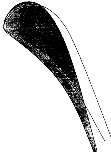
Fig. 4 : Initial (grey) and redesigned blade (—) when imposing constant outlet pressure
