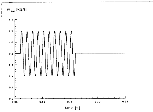
Figure 17: Oscillations in fuel flow-rate
