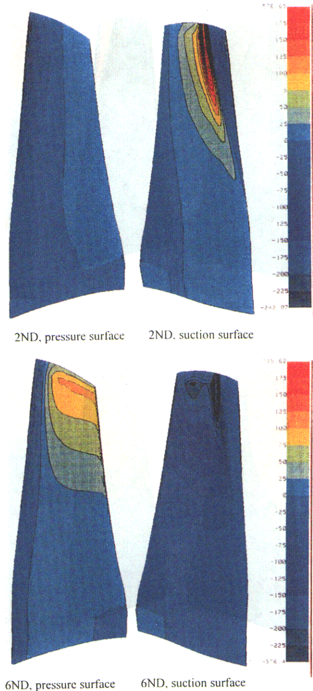
Figure 6: Worksum, wide chord fan blade
