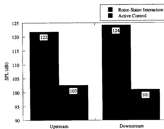
Figure 10. Simultaneous up &amp; downstream control
