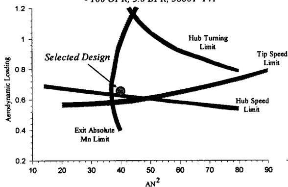
Figure 11 - GSA High Pressure Spool Design Space
