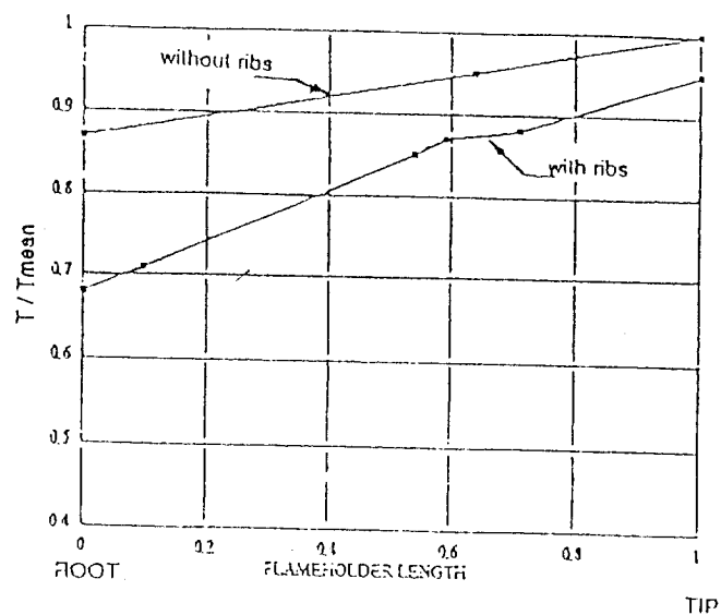
Figs. 9a - Flameholder Cooling Duct with 60° oriented Turbulence Promoters Fig. 9b - Flameholder Temperature : Effect of Turbulence Promoters
