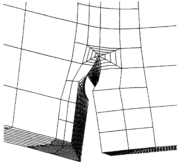
Figure 15. Crack propagation after 70 iterations.
