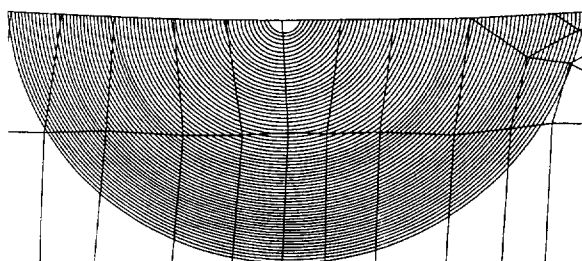
Figure 11. Crack propagation in the fir tree notch.
