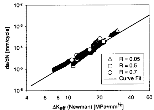
Figure 5: da/dN vs. \Delta K_{eff} for René 95 at 400°C.
