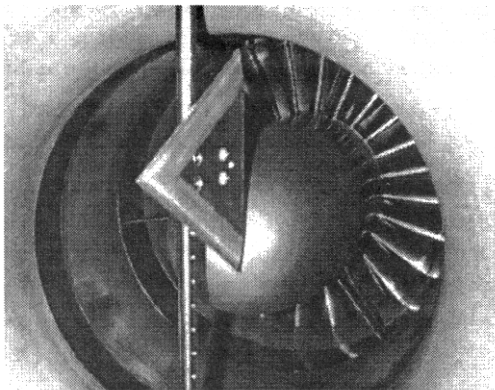
Figure 26: Delta wing for the generation of transient inlet distortions
