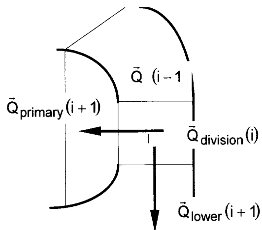
Figure 7: Reverse-flow flow-division
