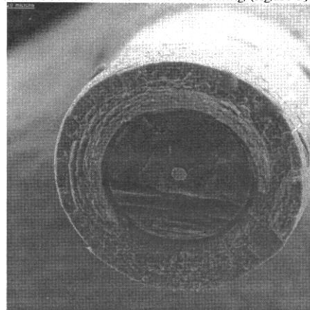
Figure 5 Matrix Coated Fibre
