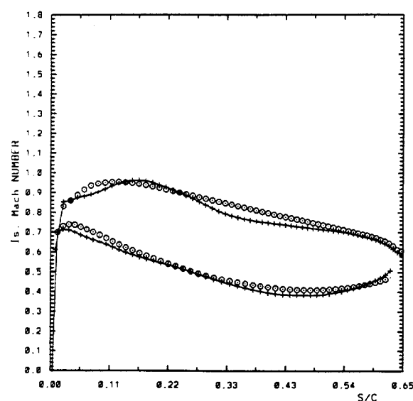
Fig. 7 : Transonic compressor rotor - Calculated (+) and target (o) Mach number distribution at shroud and hub section
