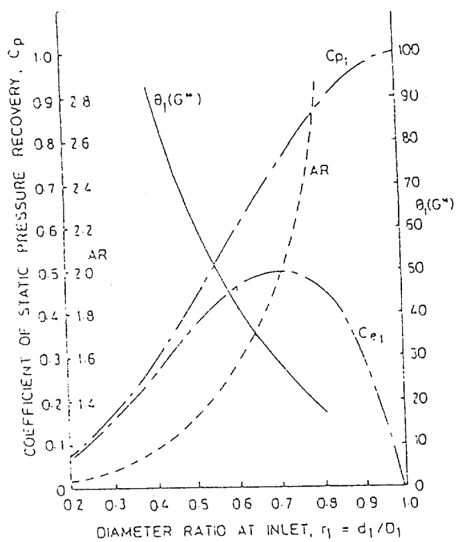
Fig. 6 - Annular Diffuser Pressure Recovery Plot
