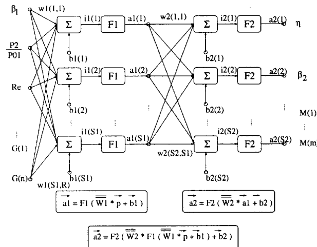
Fig. 4 : A 2-layer artificial neural network
