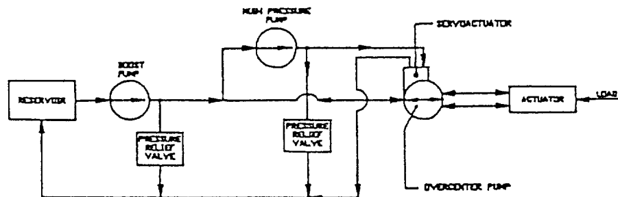
d – Pump controlled system
