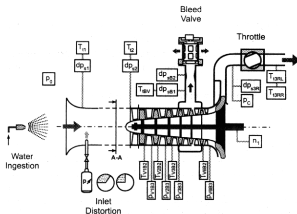
Figure 1: Compressor and facility set up
