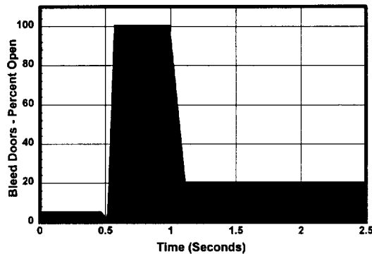
Figure 9. Bleed Bypass Doors Percent Open as a Function of Time
