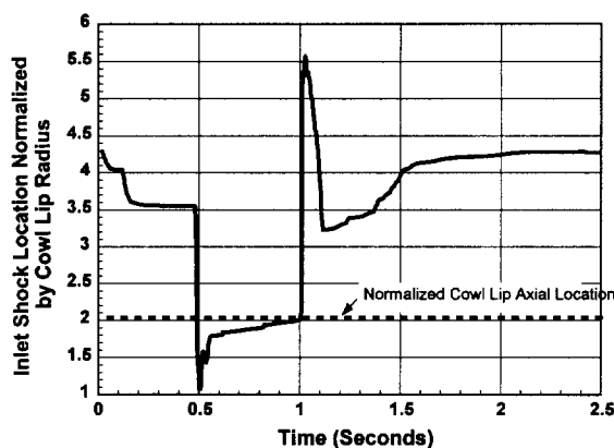
Figure 17. Inlet Shock Location Normalized by Cowl Lip Radius
