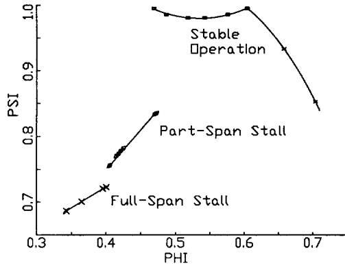
Figure 11: Characteristics of the various operating modes
