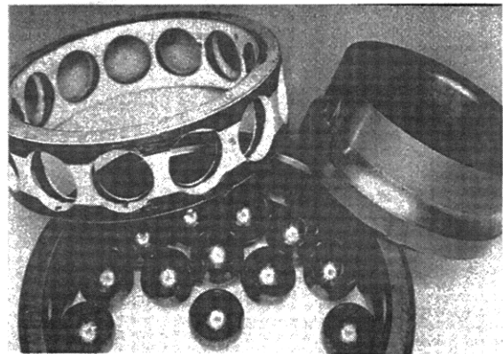
Figure 7. Condition of the test bearing after nineteen hours of testing at 425°C outer race temperature, 31,000 shaft rpm, and 445 N axial load. The rolling elements and bearing race are still in good shape. There is considerable wear in the sliding surfaces of the cage.
