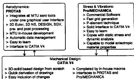
Figure 8: The Tools used in the Design Process
