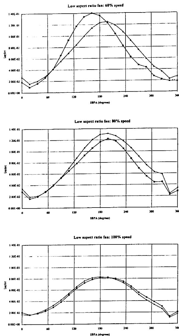
Figure 9: Stability analysis results, low aspect ratio fan
