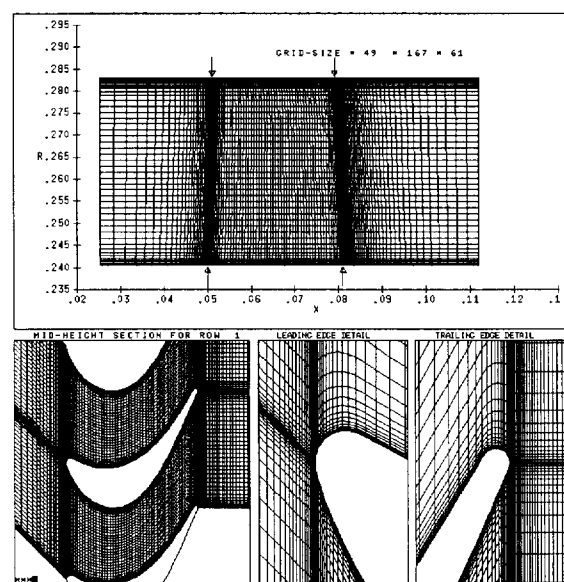
Figure 1 : JA63 Fine Grid. 167 x 49 x 61
