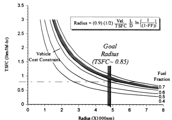
Figure 5 - Global Strike Aircraft Sensitivity Analysis
