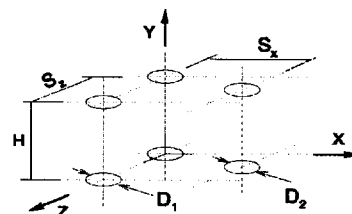
Fig. 4.1: Geometrical parameters defining an array with two rows.
