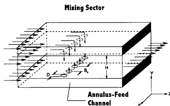
Fig. 2.1: Experimental model of RQL mixing section with geometrical parameters
