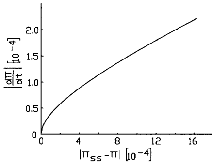
Figure 12: Transient post-stall compressor response
