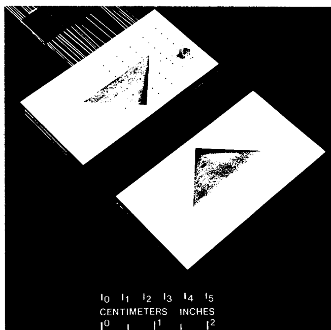
Fig. 7 A cavity supersonic vortex generator test article [7].
