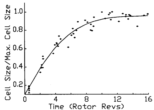
Figure 9: Time history of the cell size after stall initiation
