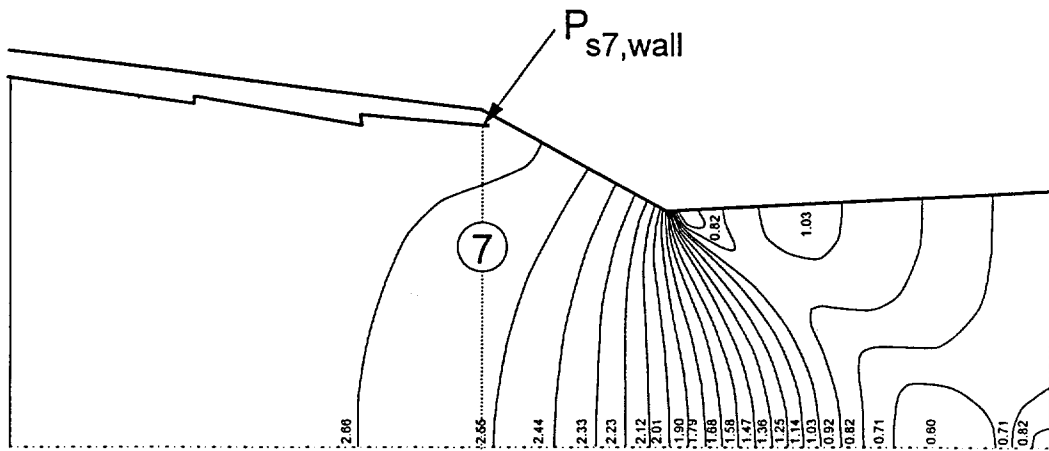
Fig. 4 Static pressure field at the nozzle inlet from CFD calculations
