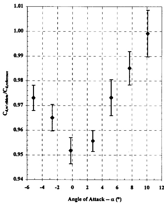
(c) Drag Ratio, Configurations B and D
