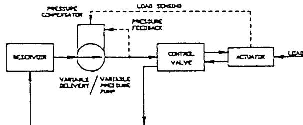
c – Valve controlled system – variable delivery pump – variable pressure
