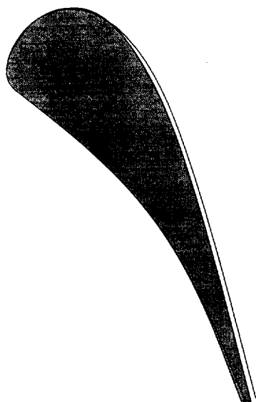
Fig. 5 : Initial (grey) and redesigned blade (—) for constant mass flow
