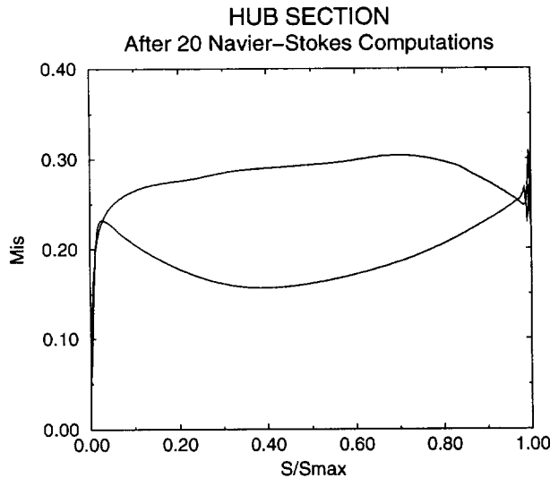
Fig. 11 : Mach number distributions on the blade surface
