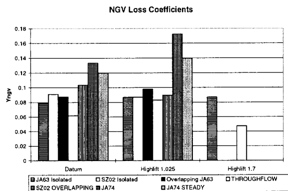
Figure 9 : Pressure Loss Coefficients, Datum and Highlift NGVs.
