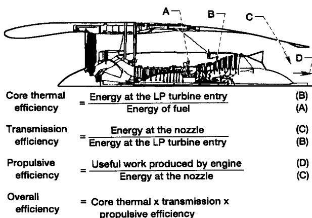
Figure 3.—Breakdown of engine efficiencies (Smith, 1993).
