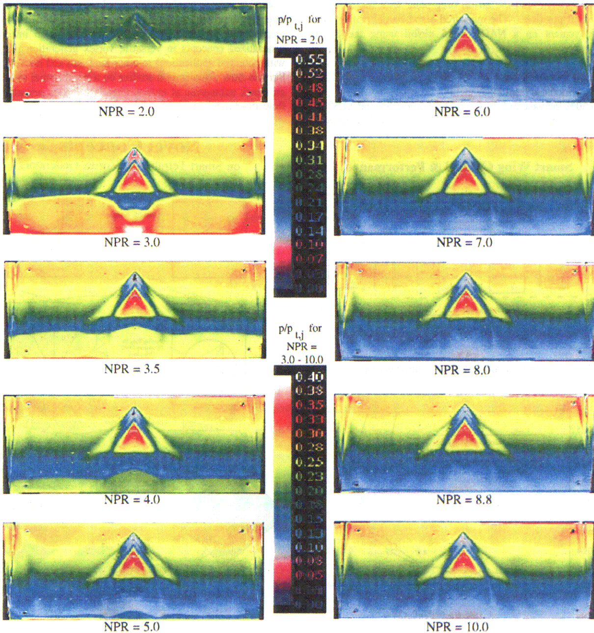
Fig. 8 Pressure sensitive paint study of a supersonic VG [8]
