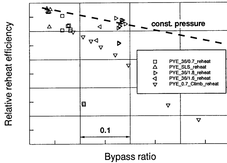
Fig. 13b Relative reheat efficiency: correlation with bypass ratio. Line is for constant pressure and fuel-air-ratio
