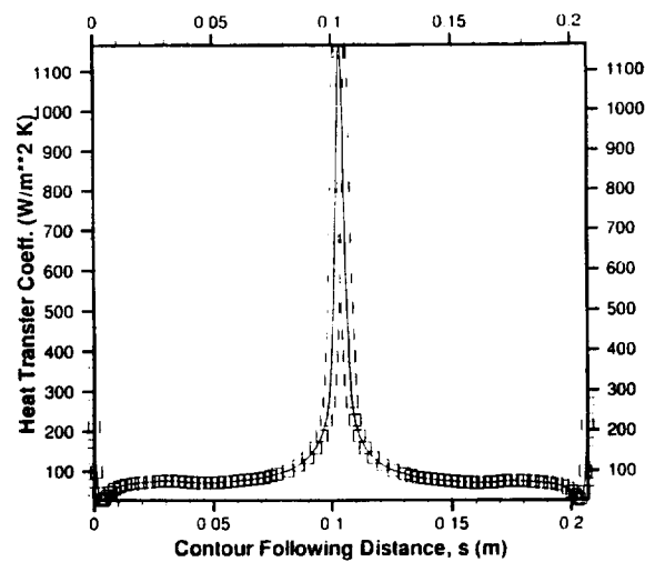
Fig. 15 Heat transfer coefficients on the external surface of the symmetric strut airfoil computed by a Navier-Stokes solver and specified as boundary conditions during thermal optimization.
