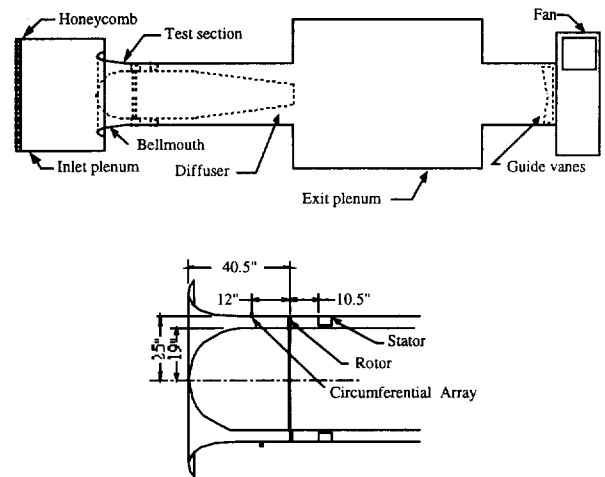
Figure 4. Purdue Annular Cascade Facility
