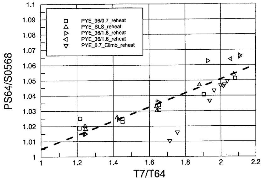
Fig. 14 Correlation between the calculated mixer pressure P_{s64} and the measured pressure S0568 (on the liner) in reheat operation
