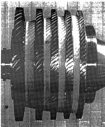
Figure 3: EJ200 5-Stage HP-Compressor, Bladed Rotor
