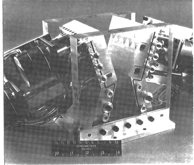
a) smart nozzle hardware assembly (4 stepper motors)
