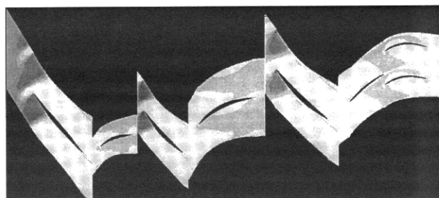
Fig. 10 3D multistage viscous analysis for PW150 low pressure compressor
