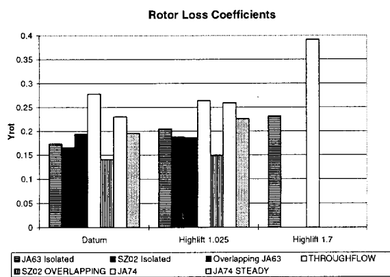
Figure 10 : Pressure Loss Coefficients, Datum and Highlift Rotors.
