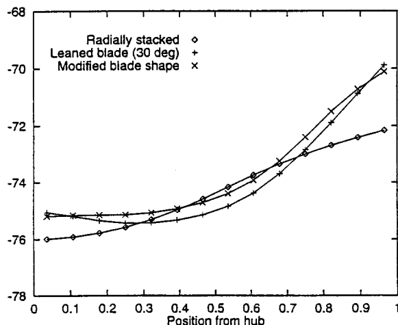
Fig. 15 : Spanwise variation of outlet flow angle
