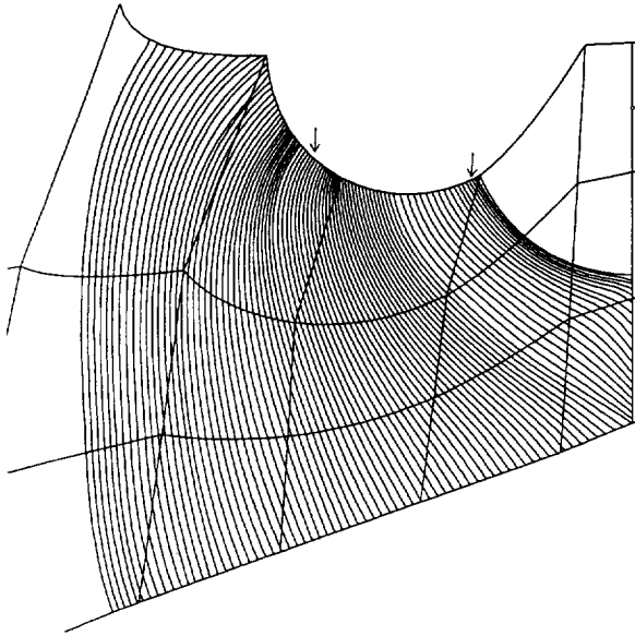
Figure 3. Crack propagation at the locking plate slot.
