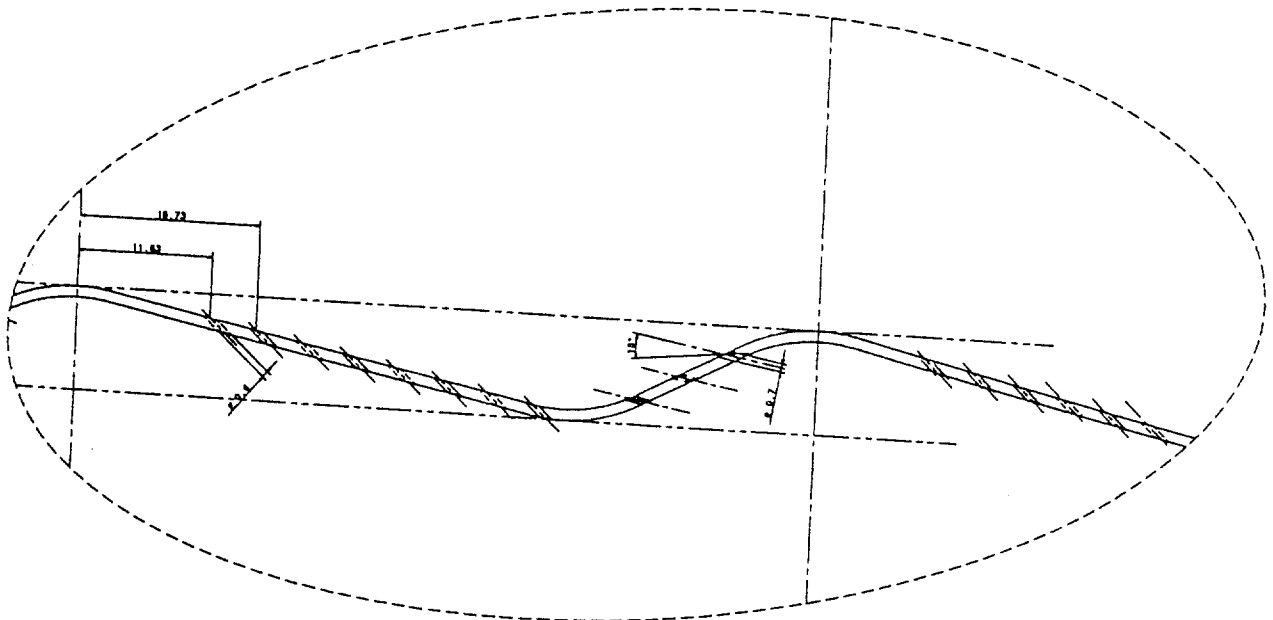
Fig. 4 - Corrugated ("Wavy") Heat Shield Cooling Holes
