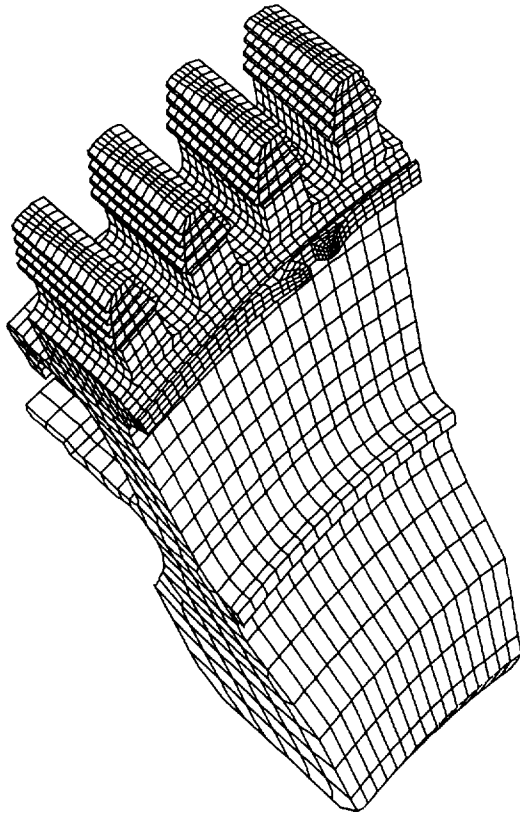
Figure 1. Aircraft engine disk segment
