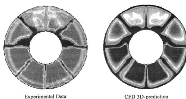
Fig. 9 PW150 intake total pressure profiles
