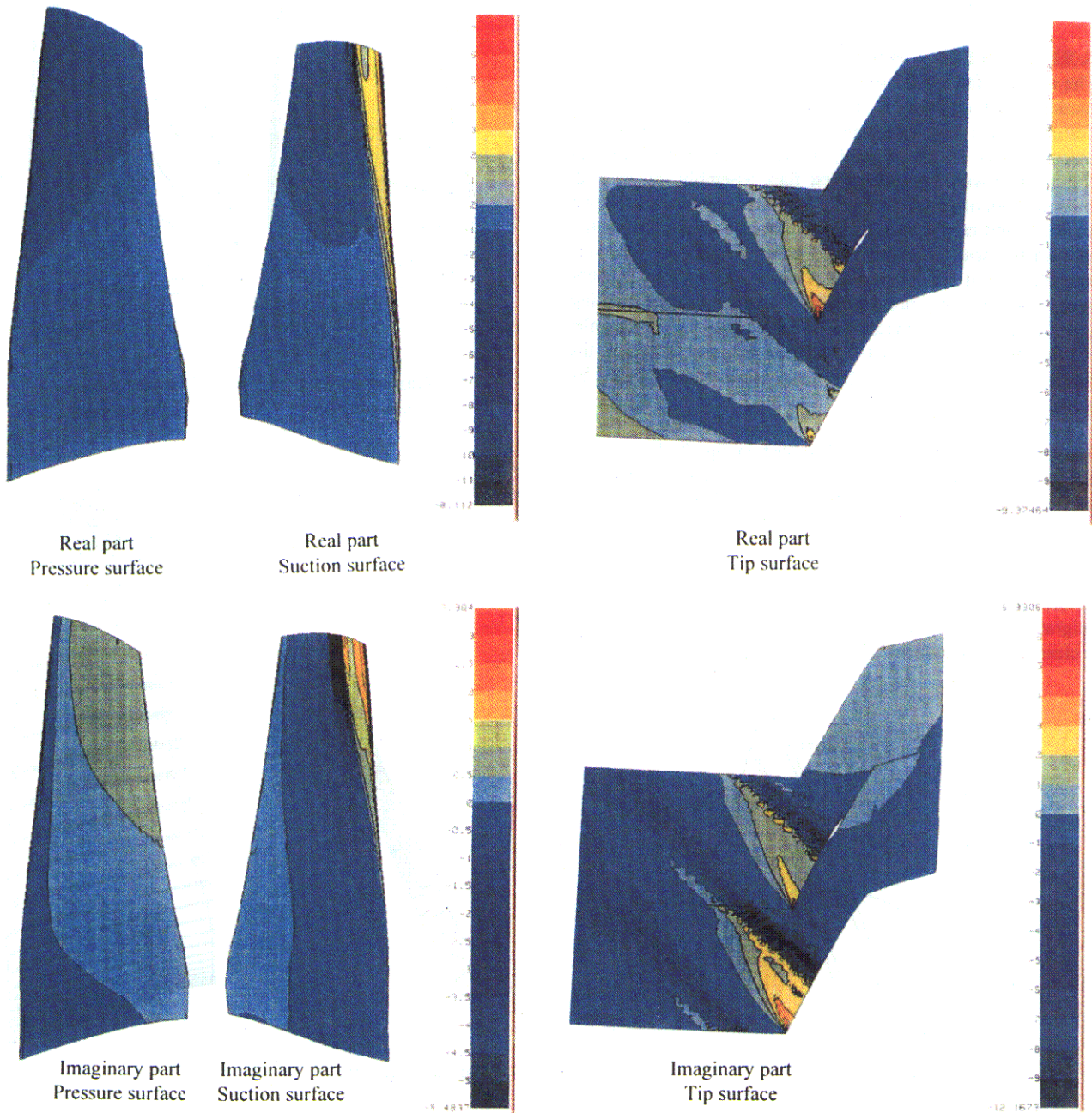
Figure 4: Real and imaginary components of pressure perturbation, wide chord fan blade, 2ND
