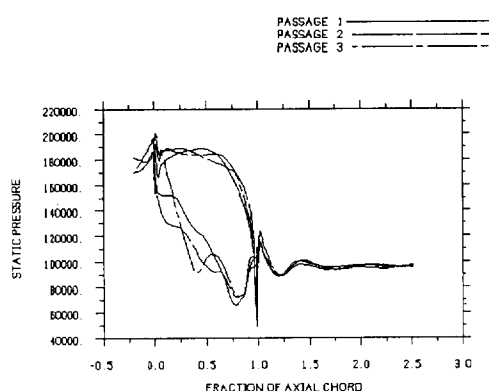
Figure 20 : Datum Mid-Span Unsteady Static Pressure Plots
