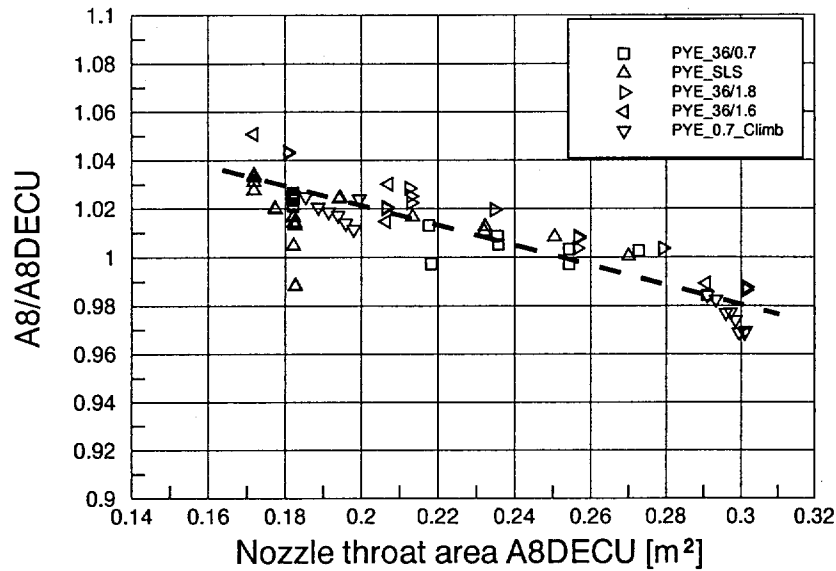
Fig. 15a Deviation between the analysed nozzle area A_8 and the control system input A_{8,DECU} correlated with nozzle position
