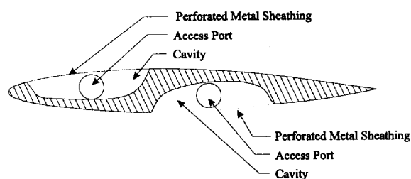
Figure 9. Active airfoil chordwise cross-section
