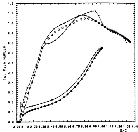
Fig. 3 : Mach number distribution on the original blade (+), the imposed target Mach number distribution (o) and the one on the blade obtained after 600 iterations of the design procedure with fixed outlet static pressure (x)
