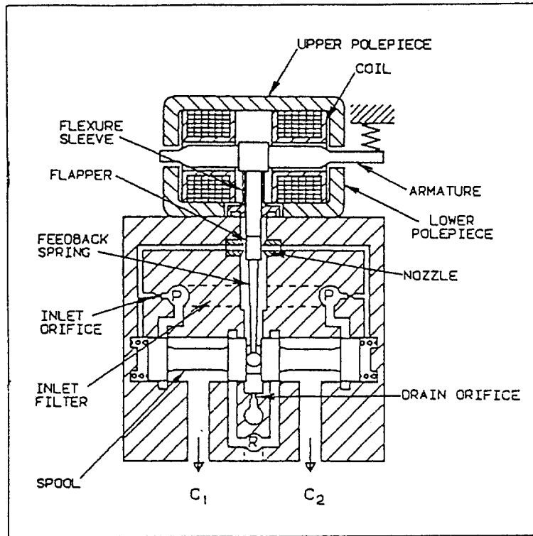
Fig. 6 - VACU 4-way Servovalve Schematic
