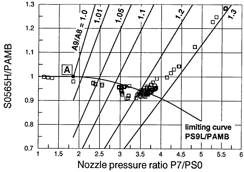
Fig. 10 Measured static pressure near to the nozzle exit
