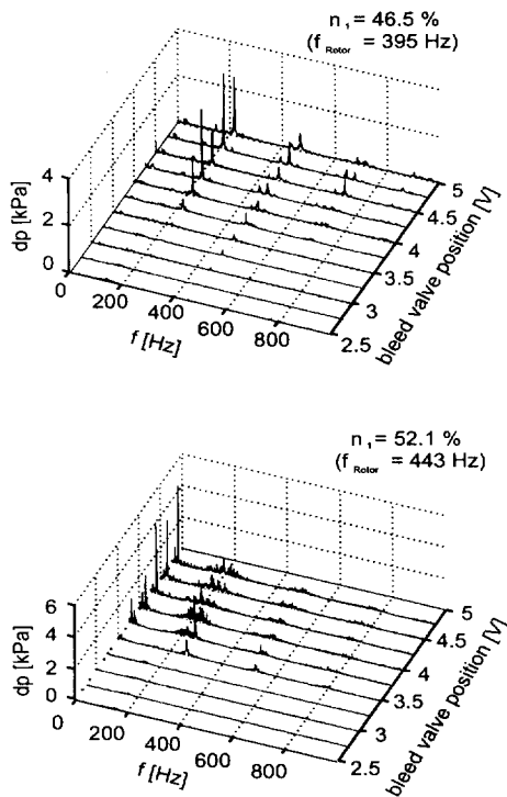
Figure 9: FFT-Analysis of the axial flow compressor outlet pressure
