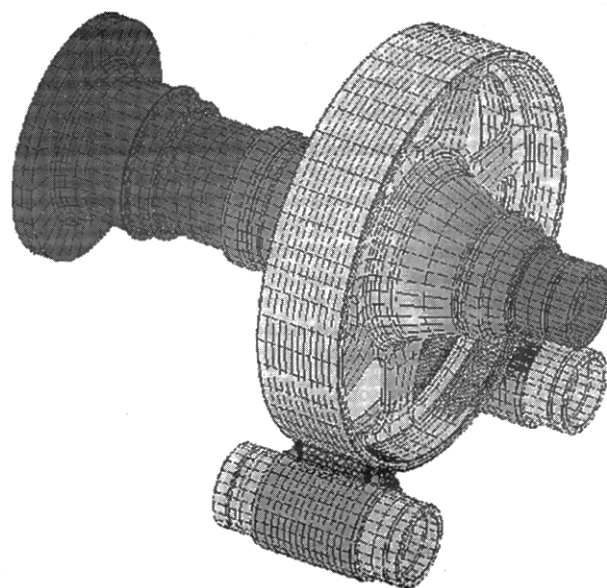
Fig. 21 PW100 gearbox second stage finite element analysis
