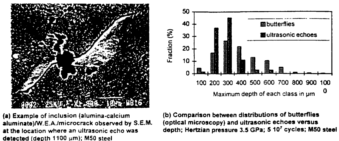
Figure 3 : Butterflies and ultrasonic echoes versus depth
