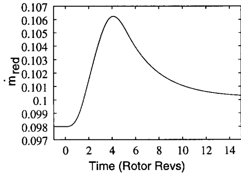
Figure 22: Mass flow transient of the experiment shown in Fig. 19 (mathematical model)
