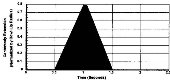
Figure 10. Centerbody Extension (Values Normalized by Cowl Lip Radius)
