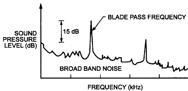
Figure 2. Typical turbomachine noise spectrum
