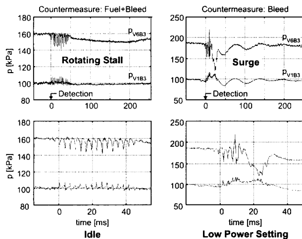
Figure 18: Rotating stall and surge detection
