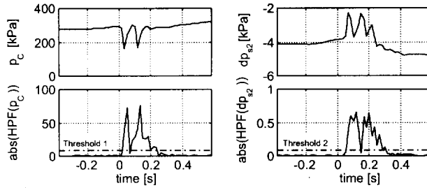
Figure 17: High-pass filtered pressure signals during surge
