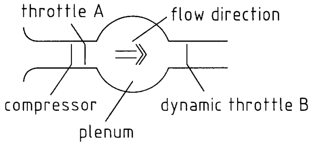
Figure 2: Schematic overview of the compression system
