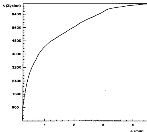
Figure 8. Cycles versus maximal crack length
