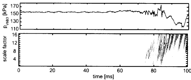
Figure 12: Wavelet analysis of compressor stall
