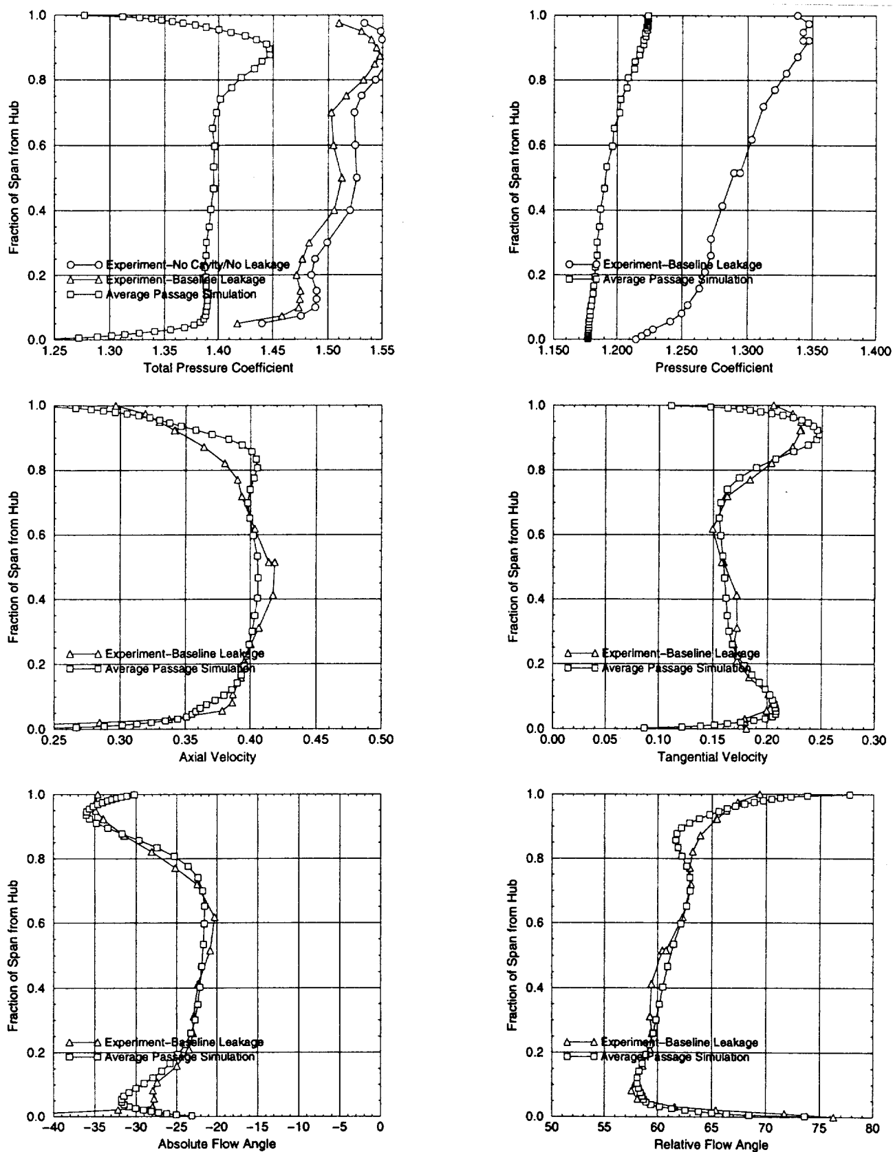
Fig. 6. Axisymmetric flow variables at Station 4.0.
