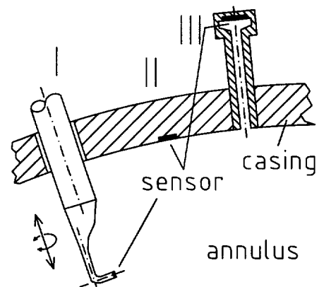
Figure 5: Dynamic pressure probes
