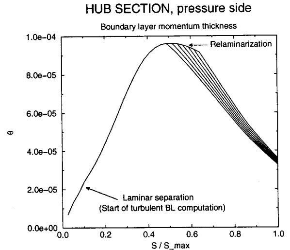
Fig. 13 : Boundary layer momentum thickness (pressure side)
