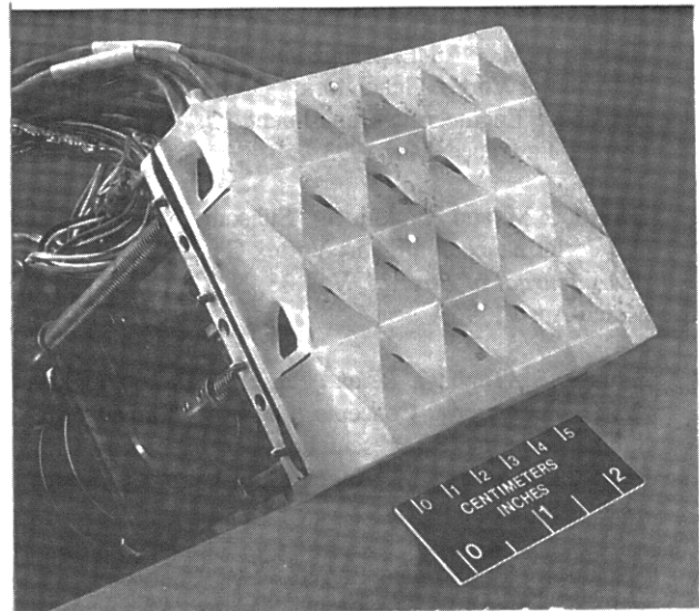
b) Four rows of VGs and 8 Kulite transducers
