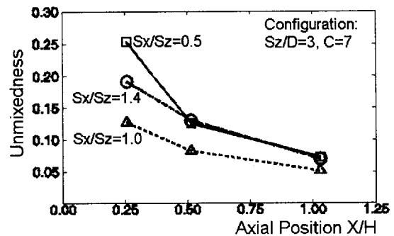
Fig. 4.4: Effect of row spacing on mixture homogeneity
