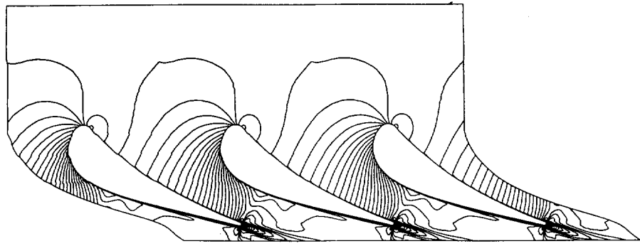
Fig. 8 Static pressure contours for the viscous stator domain
