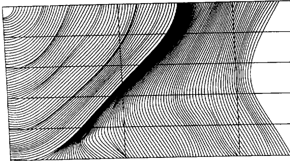
Figure 7. Crack propagation in the platform.
