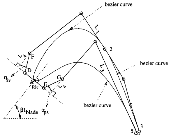
Fig. 3 : Geometry model : Bézier curves
