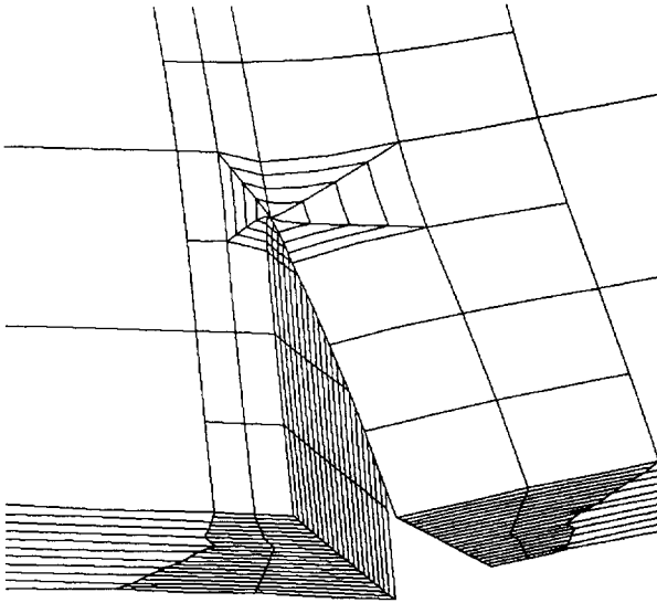
Figure 14. View of the crack tip region.
