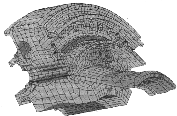
Fig. 18 PW100 high turbine centrifugal stresses
