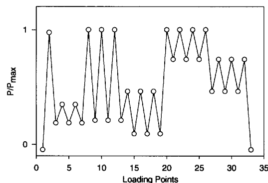
Figure 6c: Experimental Loading History 3 (LS 3).
