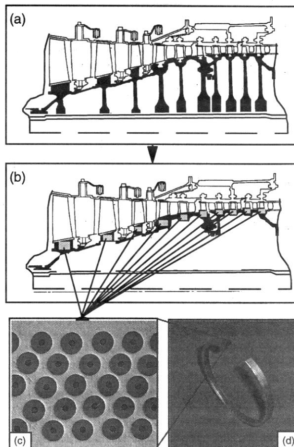
Fig. 13: Compressor design with TMCs; (a) conventional compressor design, (b) bling (bladed ring) design with TMCs, (c, d) fiber distribution in a TMC ring produced via the matrix coated fiber technique.
