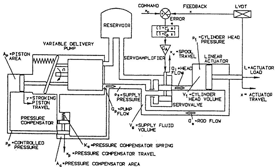
Fig. 7a - NACU Diagram for Linear Model Calculations
