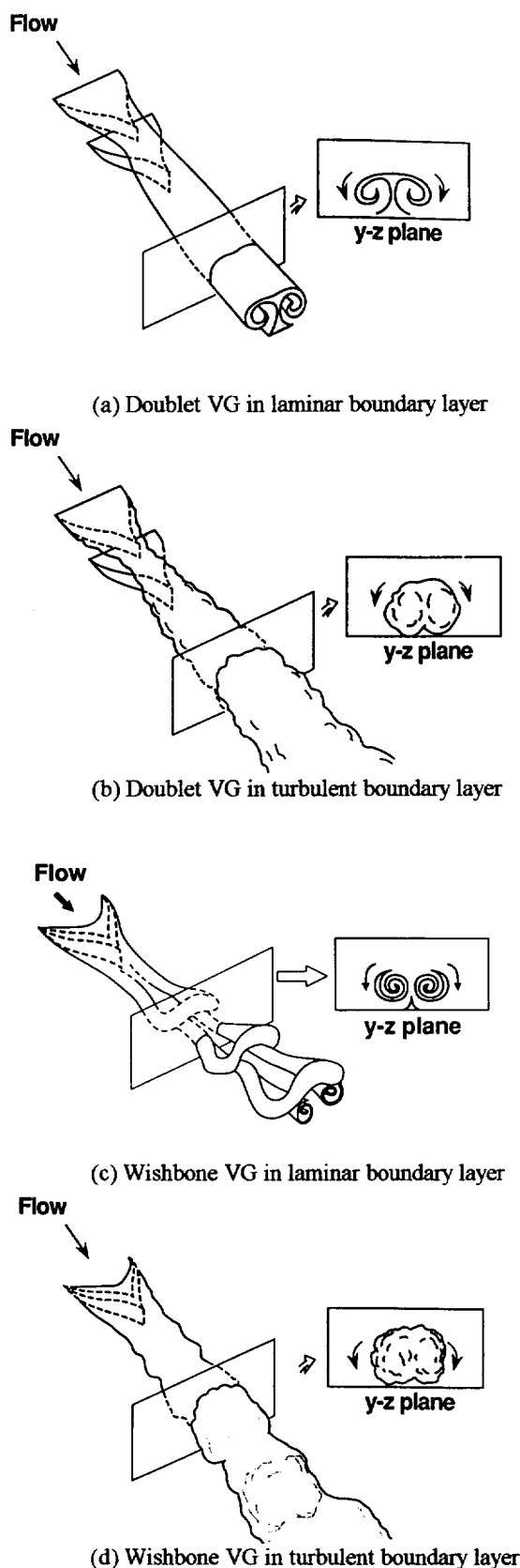
Fig. 6 Flow structure downstream of doublet and wishbone vortex generators [17].
