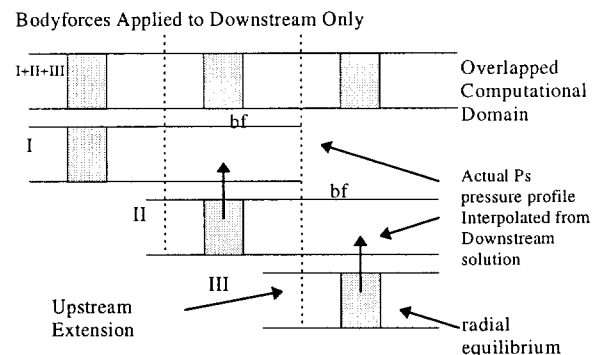
Figure 3 : Illustration of Overlapping Grid Principle
