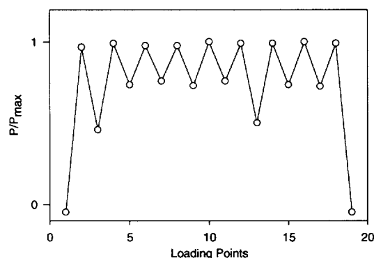
Figure 6a: Experimental Loading History 1 (LS 1).
