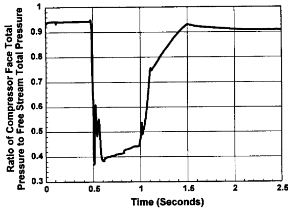
Figure 14. Model Predictions: Ratio of Compressor Face Total Pressure to Free Stream Total Pressure
