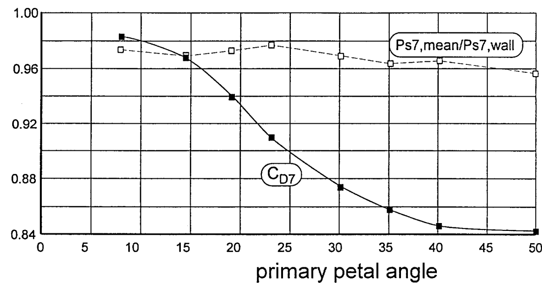
Fig. 5 CFD results for the nozzle inlet blockage coefficient C_{D7} and for P_{s7,mean}/P_{s7,wall} (ref. ITP)
