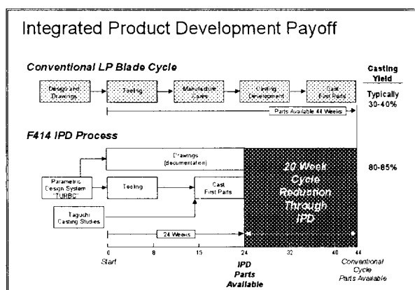
Concurrent Engineering of LPT Blade (Figure 4)
