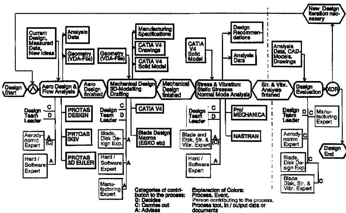
Figure 10: Advanced Multidisciplinary Process Visualization
