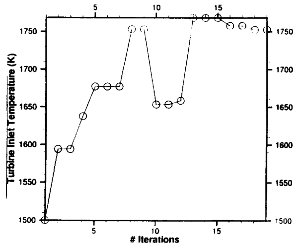
Fig. 16 Inlet hot gas temperature maximization history for the symmetric strut airfoil.
