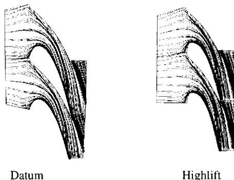
Figure 12 : NGV Endwall Streamlines - Hub.
