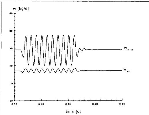
Figure 18: Effect in mass flow-rates
