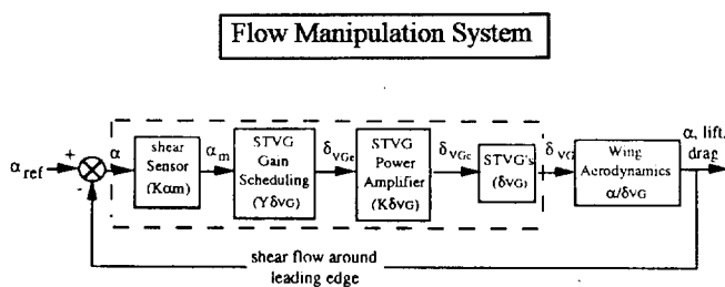
a) schematic of the STVG control system
