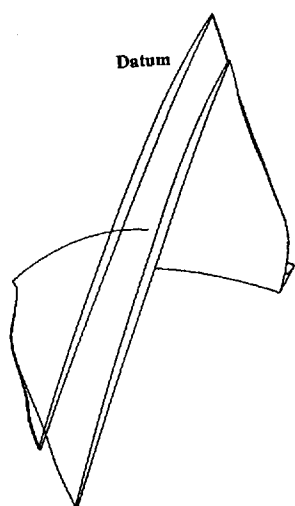
Figure 1: First flap modeshape, wide chord fan blade
