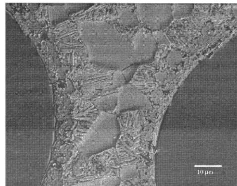
Figure 10 Extreme Interface Reaction
