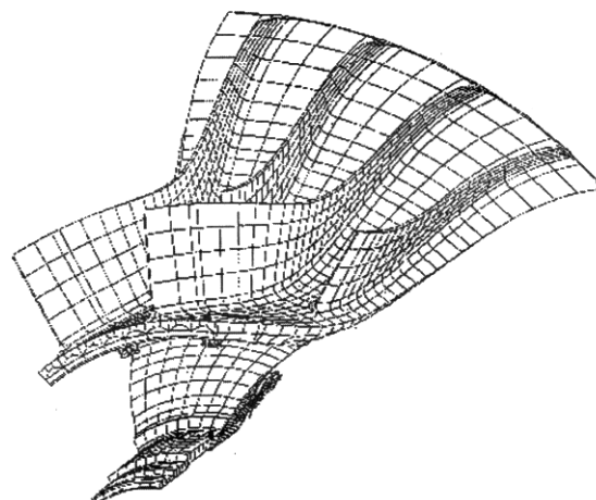
Fig. 11 3D finite element model of PW127 impeller
