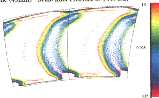
Figure 25 : Total Pressure Contours at the Highlift NGV Exit Plane (49mm) - Scale Inlet Pressure to 15% loss
