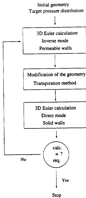
Fig. 1 : Flow chart of moving wall inverse design method
