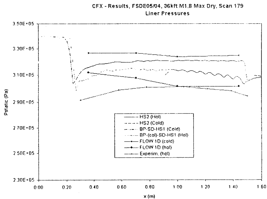
Fig. 15c - 36kft/1.8-Max Dry - CFD computed static pressure vs. Engine measured static pressure
