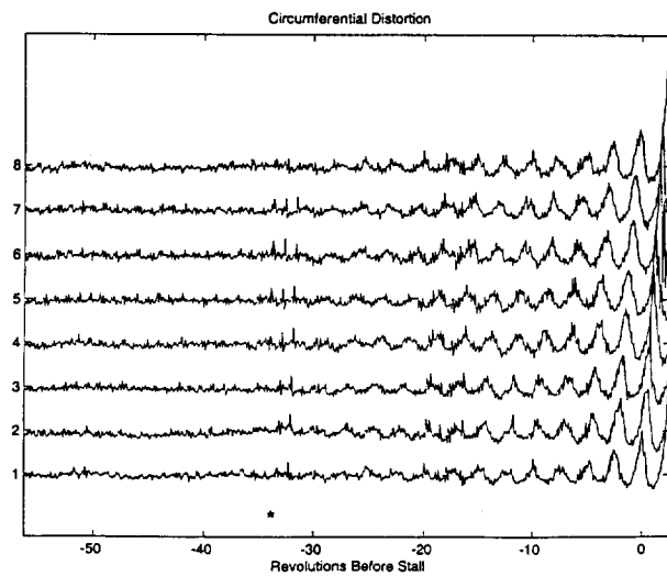
Figure 4. Pressure Traces for Circumferential Distortion
