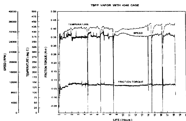
Figure 6. Experimental results for a 30 mm bore ball bearing lubricated with a tertiary-butyl phenyl phosphate lubricant delivered as a vapor at a temperature of 325°C. Test conditions: 425°C outer race temperature, 31,000 shaft rpm, and 445 N axial load.
