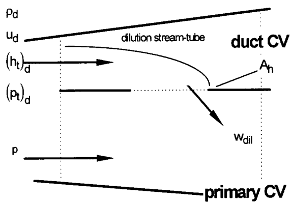
Figure 8: Dilution characteristics
