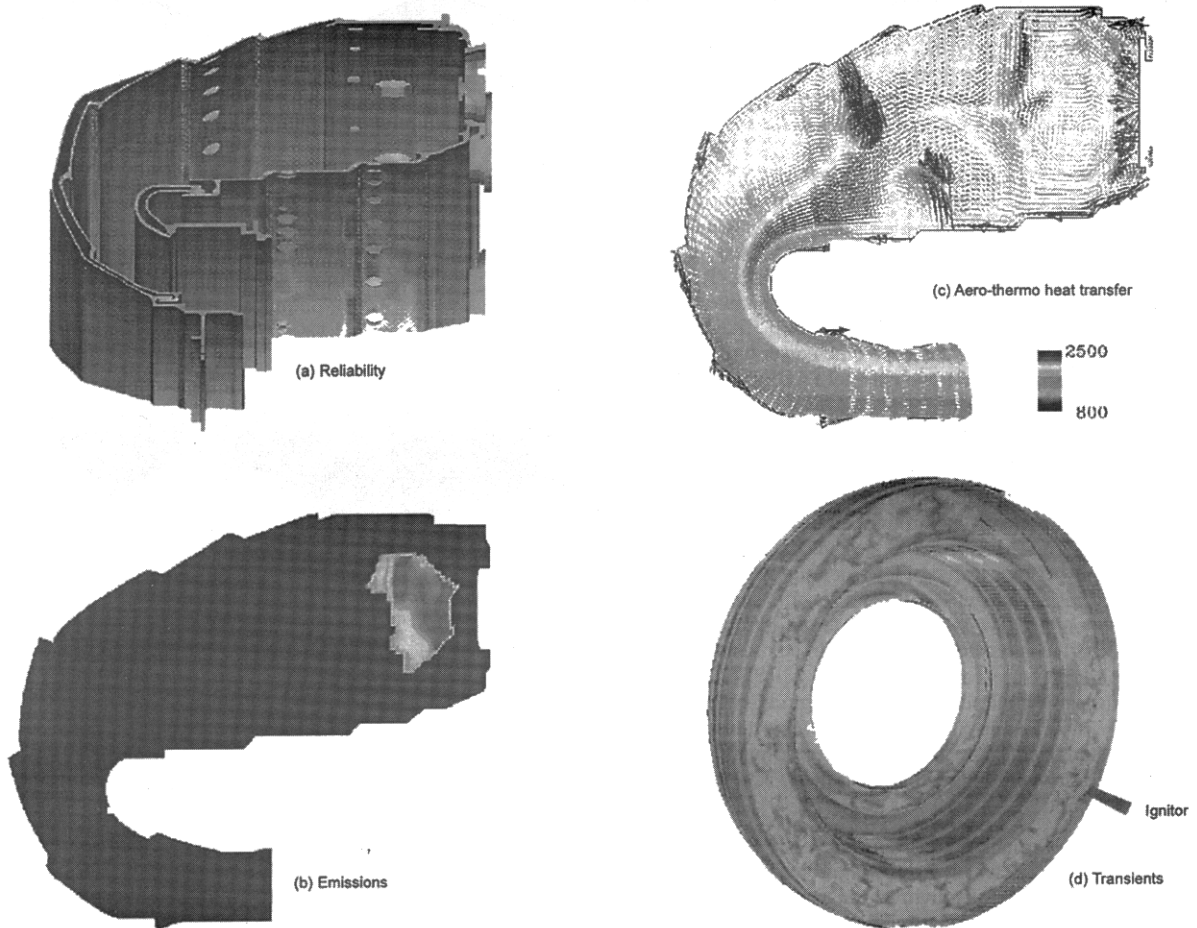
Fig. 13 PW150 combustor numerical modelling
