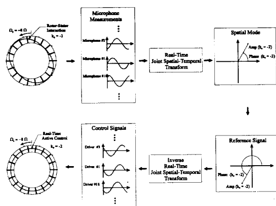
Figure 7. Active noise control system
