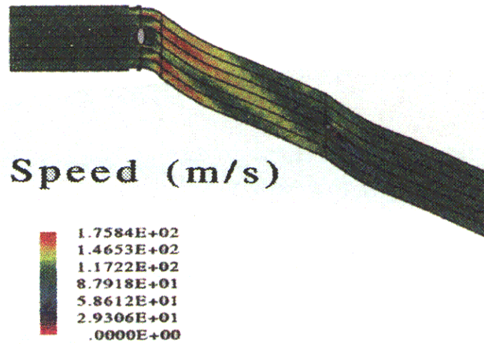
Fig. 19 - Liner Cooling Annulus - CFD computed flow velocity field
