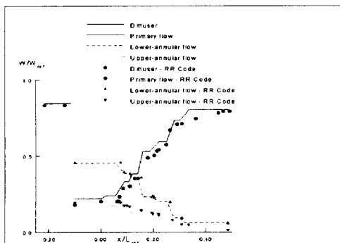
Figure 10: Total pressure - "Inviscid"
