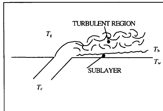
Fig.1. Schematic diagram showing turbulent region and sublayer
