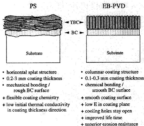
Fig. 15: A simplified comparison of properties for plasma sprayed (PS) and evaporated (EB-PVD) TBCs (schematic).
