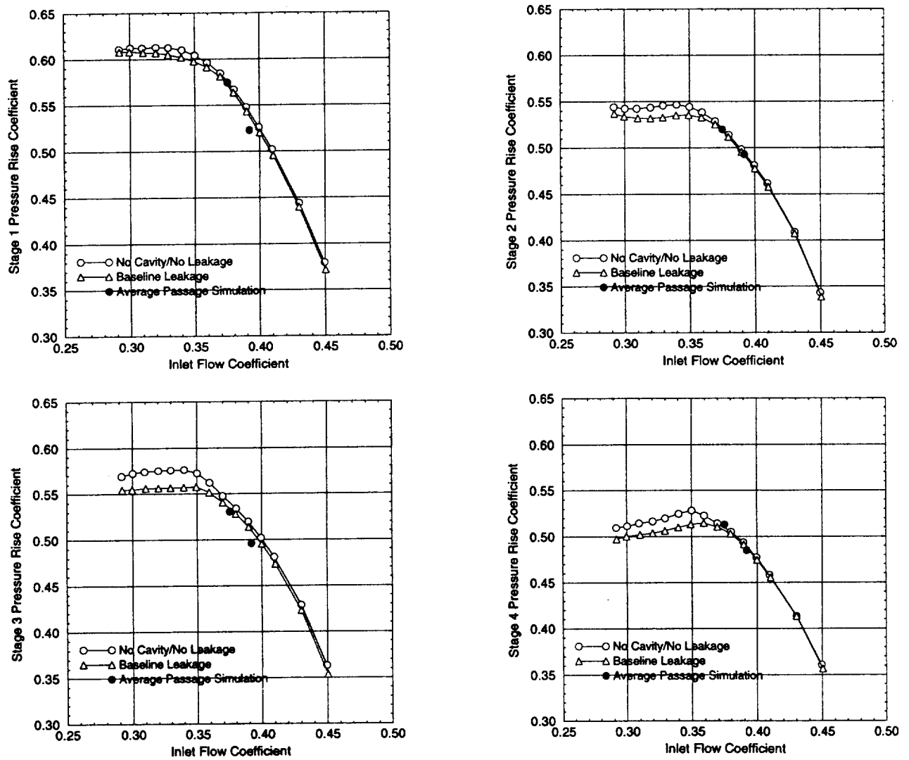
Fig. 12. Individual stage pressure rise coefficient as a function of inlet flow coefficient.
