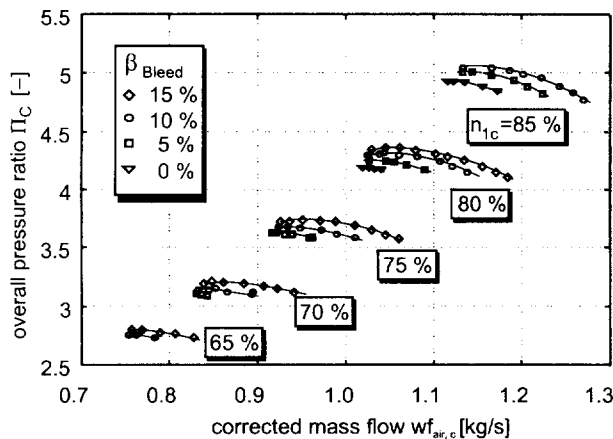
Figure 6: Measured engine compressor map
