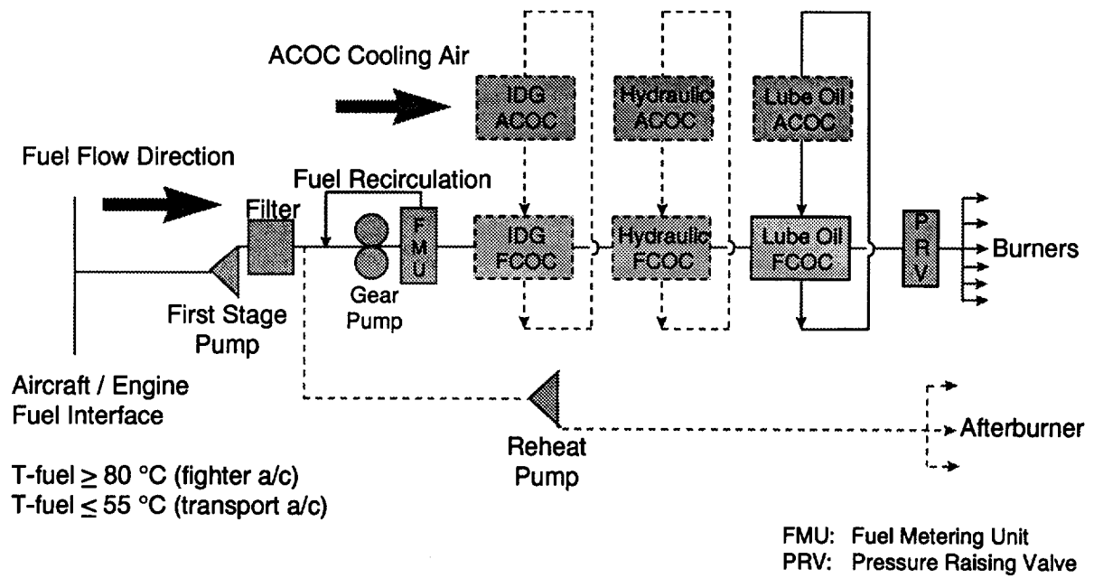
Figure 1: Heat Management System
