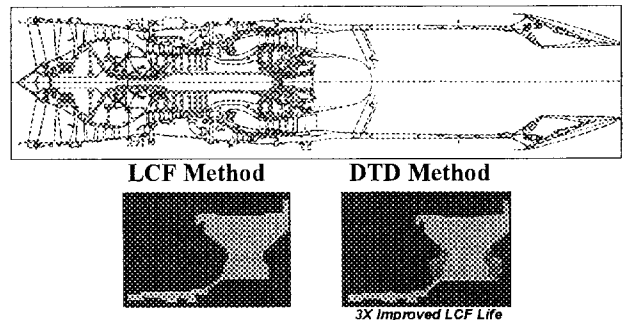
Fan Stage 1 Disk DTD Hardware (Figure 9)
