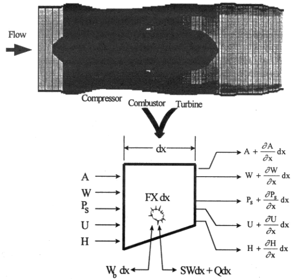
Figure 1. System Discretization into Elemental Control Volumes
