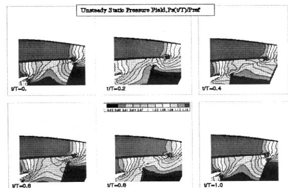
Figure 11 - Unsteady flow field, static pressure.
