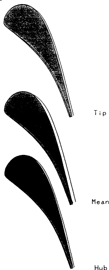
Fig. 14 : Initial (grey) and modified blade shapes
