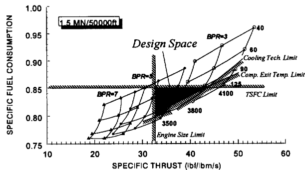
Figure 6 - GSA Uninstalled Performance Trades (With Constraints)
