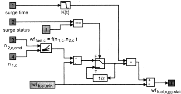
Figure 21: Control scheme of gas generator stabilization
