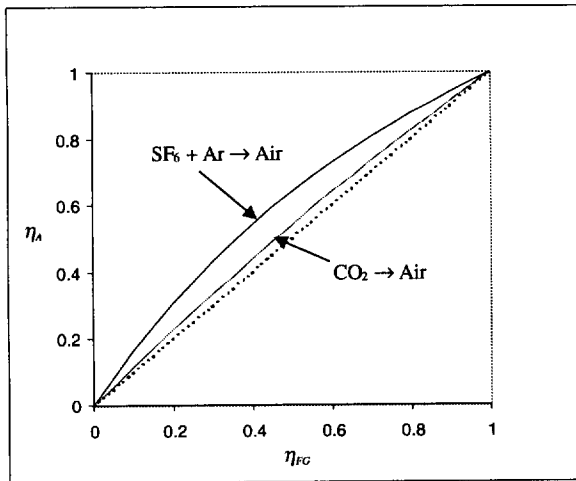
Fig.3. Film cooling effectiveness for cold air, \eta_A , versus the equivalent value for foreign gas, \eta_{FG} . Eqn (10b).
