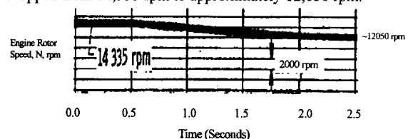
Figure 13. Test Data: Engine Shaft Rotational Speed (Choby, et al., 1971, with reference to Cole, et al., 1969)
