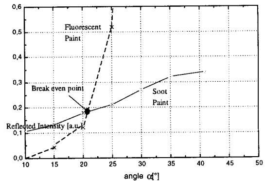
Fig. 3.3: Break even point in suppression efficiency
