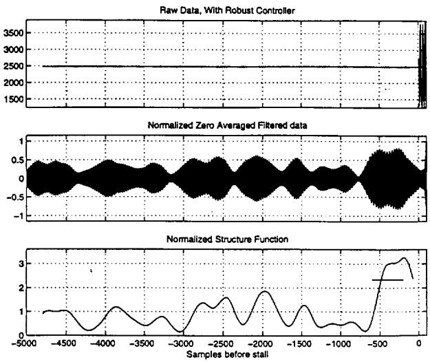
Figure 9. Structure Function Results Controlled Injection
