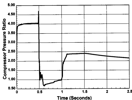
Figure 21. Compressor Pressure Ratio
