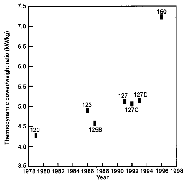
Fig. 5 PW100 specific power evolution
