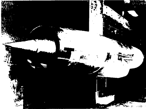
Figure 7. A 4060 Inlet and J85-13 Turbojet Installed in the LeRC 10x10 Supersonic Wind Tunnel (Calogeras, 1969)
