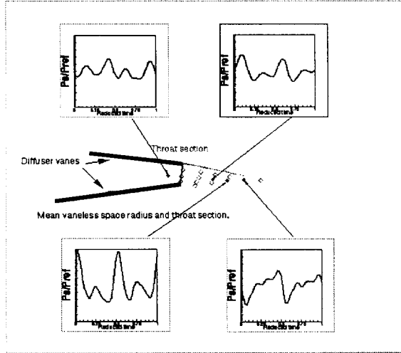
Figure 5 - Pressure evolutions (1).
