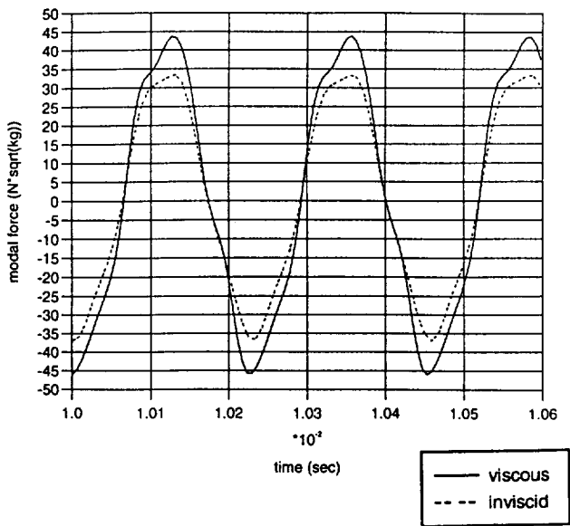
Fig. 13 Modal forces obtained from viscous and inviscid stator representations
