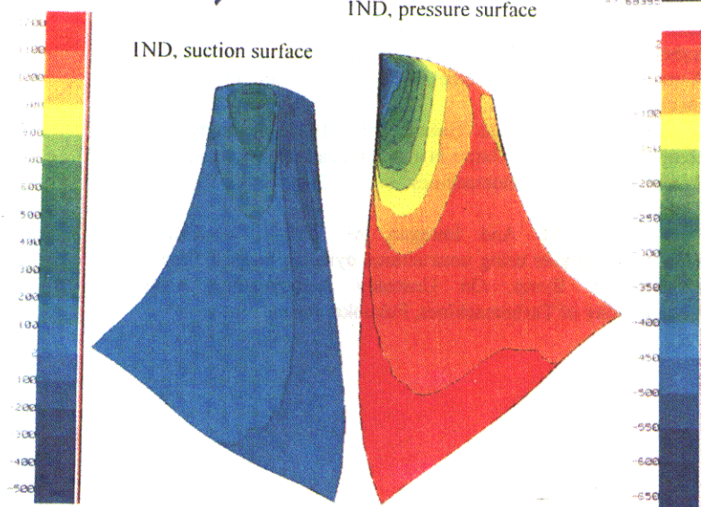
Figure 11: Worksum, low aspect ratio fan
