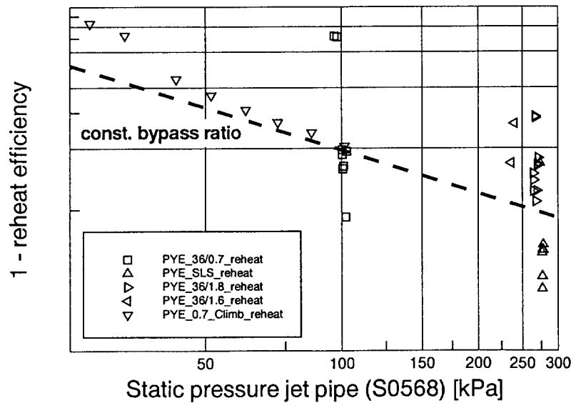
Fig. 13c Reheat efficiency: correlation with pressure. Line is for constant bypass ratio and fuel-air-ratio
