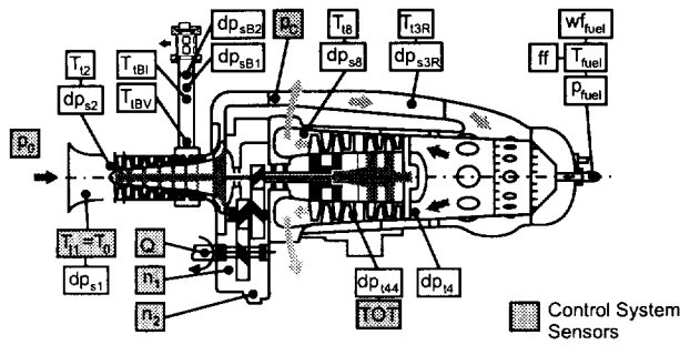
Figure 5: Engine instrumentation
