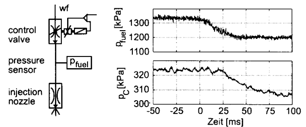
Figure 19: Reaction of the compressor pressure to the fuel flow drop
