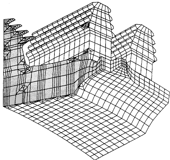
Figure 9. Crack plane before smoothing.
