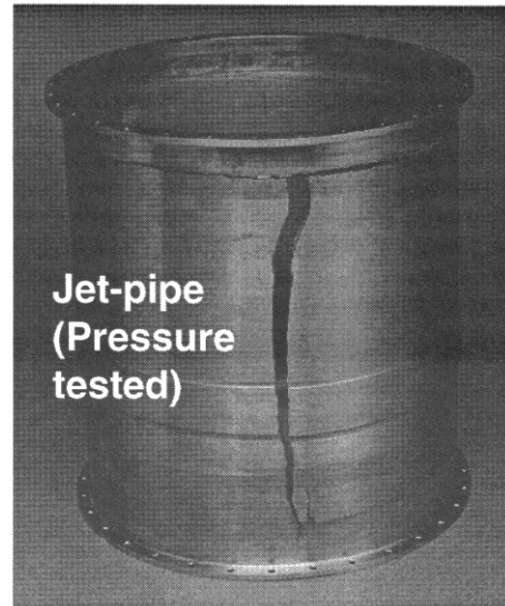
Figure 3 Successful Test of a Gem Jet Pipe
