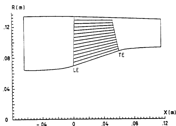
Fig. 6 : Meridional view
