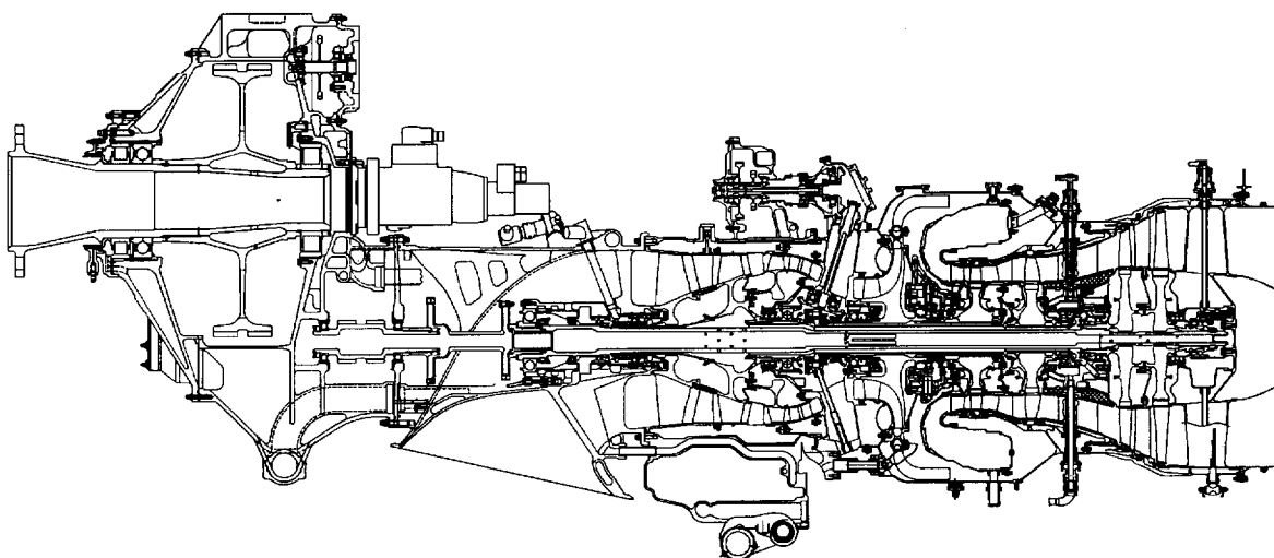
Fig. 6 PW120 gas turbine
