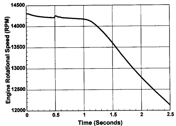
Figure 16. Model Predictions: Engine Rotational Speed
