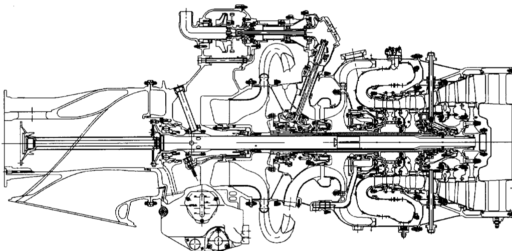
Fig. 6 PW120 gas turbine
