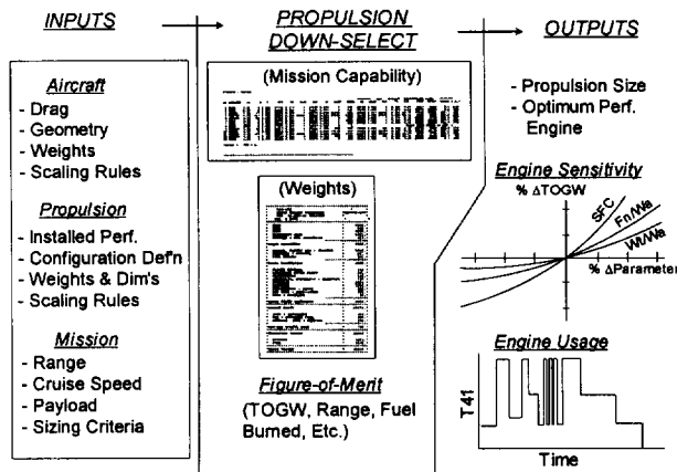
Figure 12 - Aircraft Mission Analysis
