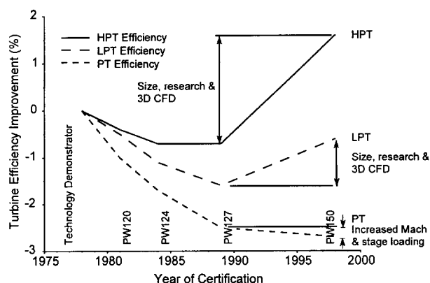
Fig. 14 Evolution of PW100 turbine efficiency
