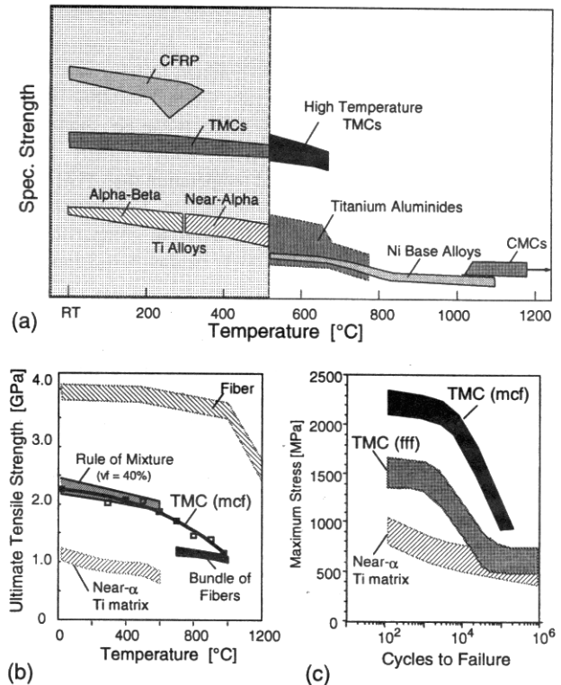
Fig. 11: Mechanical properties of TMCs: (a) specific tensile properties of TMCs and other advanced aviation materials, (b) ultimate tensile strength of TMCs produced via the matrix coated fiber technique (mcf), (c) longitudinal low cycle fatigue behavior of TMCs produced via foil/fiber/foil technique (fff) or via the matrix coated fiber technique (mcf); tests performed at room temperature ( R=0.1 , f=1\text{Hz} ).
