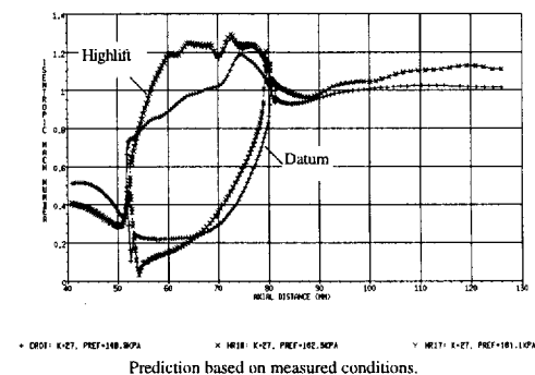
Figure 8 : Blade Surface Mach Numbers for the Datum and Highlift Rotors - Blade Mid-Section
