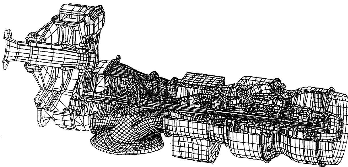
Fig. 19 PW150 full engine finite element model
