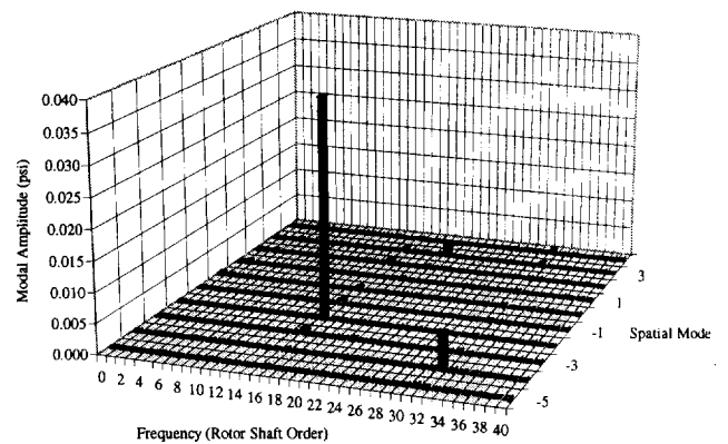
Figure 6. Rotor-stator interaction spatial modes
