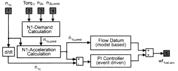
Figure 24: Flow diagram of the acceleration controller
