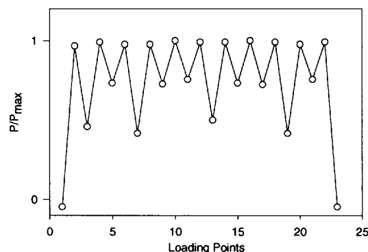
Figure 6b: Experimental Loading History 2 (LS 2).
