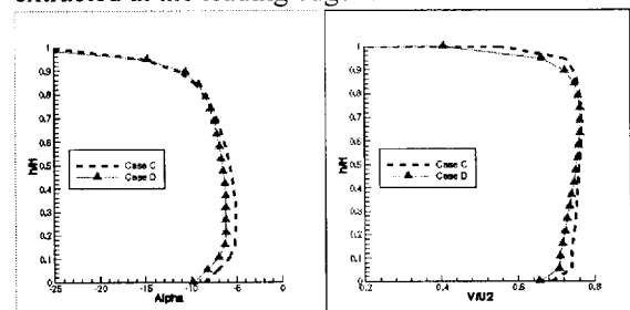
Figure 13 - Comparisons of spanwise evolutions.
