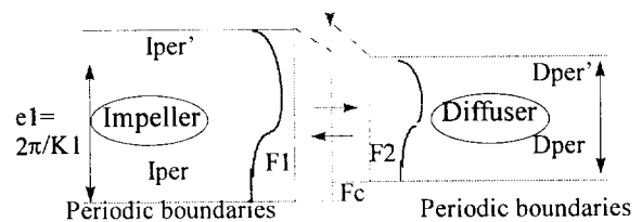
Figure 6 - Reduction of the computational domain.
