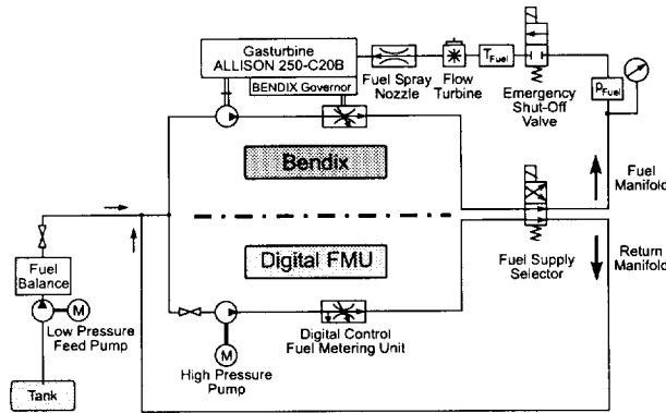
Figure 3: Schematic of the fuel system
