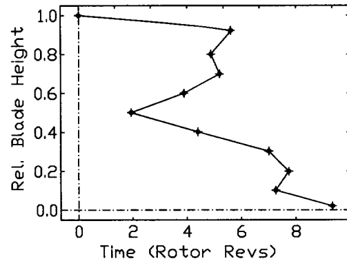
Figure 8: Delay of the stall detection at various radial locations
