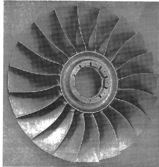
Figure 4: EJ200 3-Stage All Blisk Fan, First Rotor Stage
