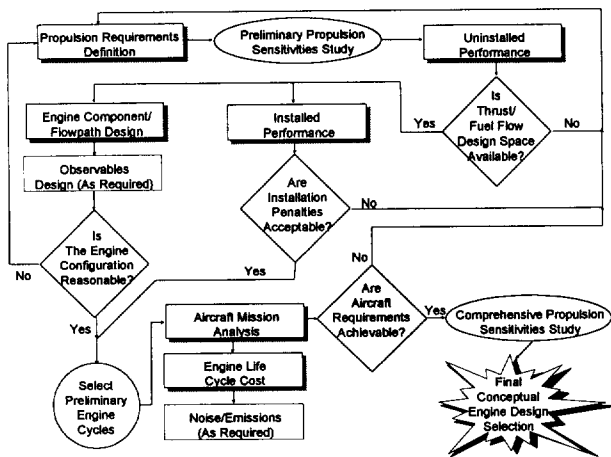
Figure 2 - Engine Conceptual Design Process
