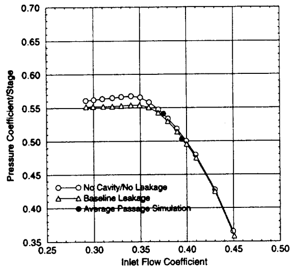
Fig. 11. Overall pressure coefficient as a function of inlet flow coefficient.
