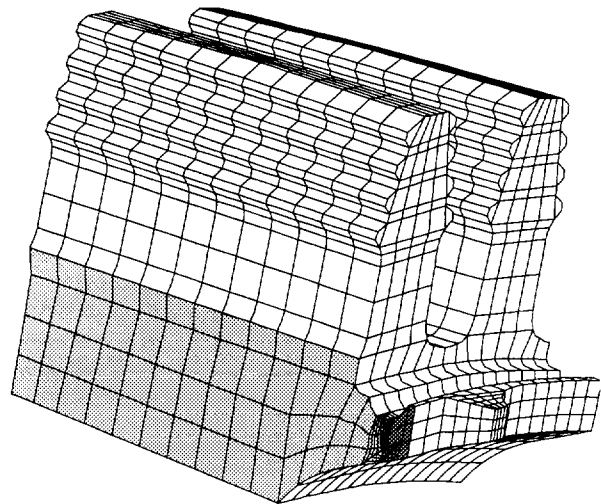
Figure 2. Details of the cracked locking plate slot
