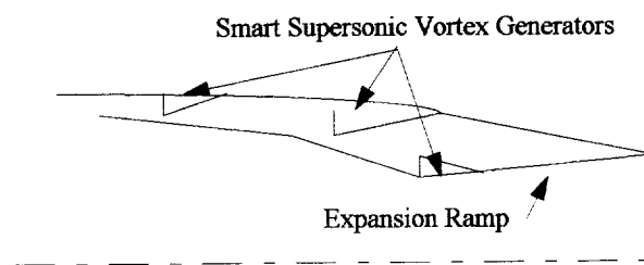
Fig. 4 Schematic of smart VGs outside (boattail) and inside a C-D supersonic nozzle.
