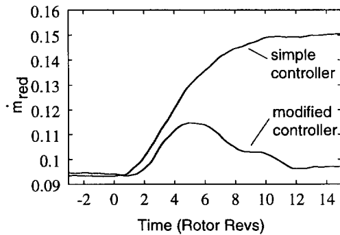
Figure 23: Measured mass flow transients from the experiments shown in Figs 18 and 19
