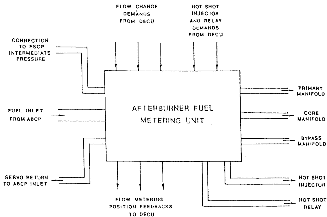
Fig. 5 - Afterburner Fuel Metering Unit Interface
