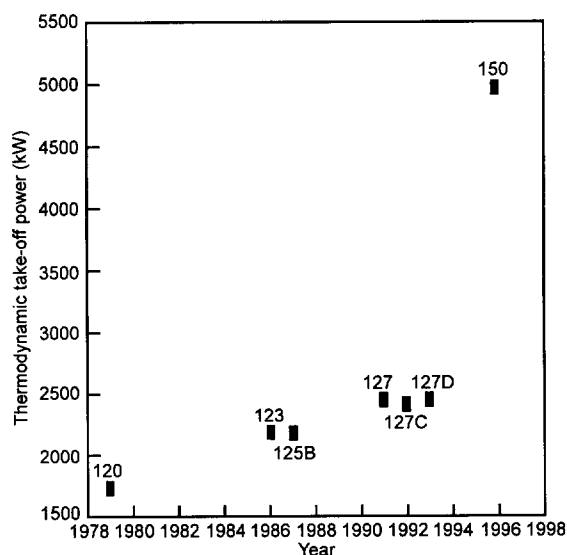
Fig. 3 PW100 power growth
