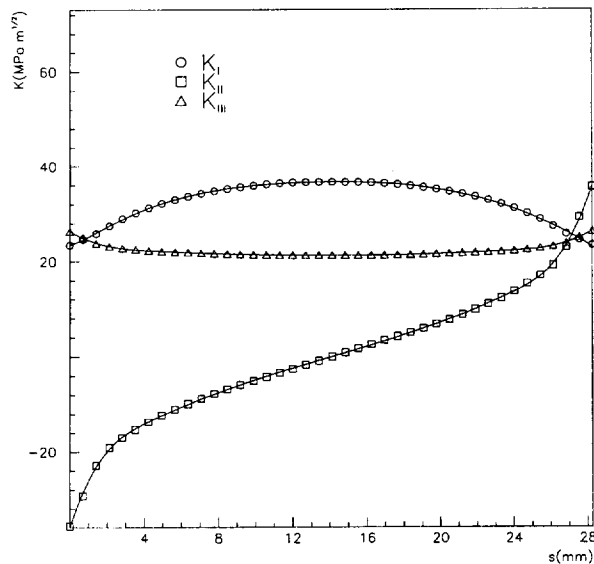
Figure 16. K-distribution along the initial front.
