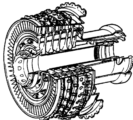
Figure 1: RB199 6-Stage HP-Compressor
